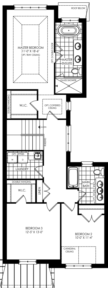
SECOND FLOOR PLAN ELEV. 'B'
