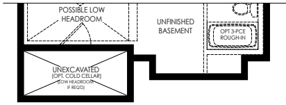
PARTIAL BASEMENT PLAN ELEV. 'D'
