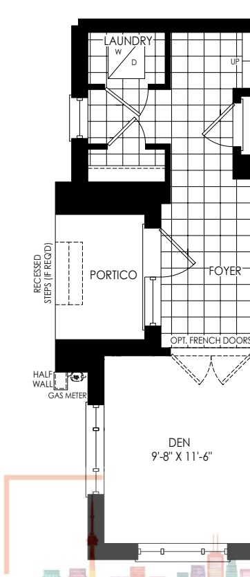
PARTIAL GROUND FLOOR PLAN ELEV. 'WC5'
