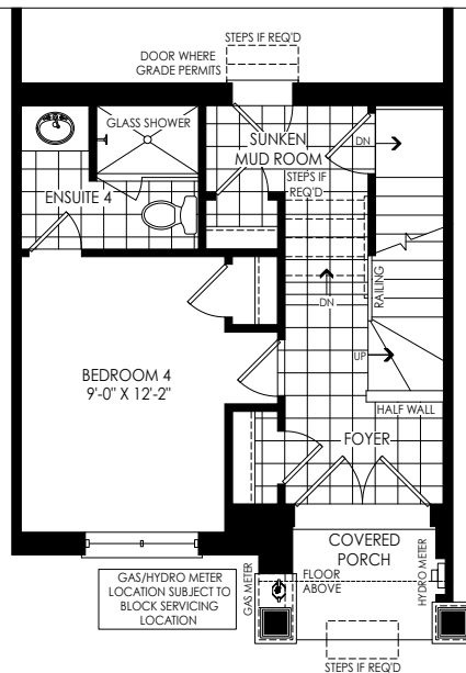
PARTIAL OPT. GROUND FLOOR PLAN W/ 4 BEDROOMS ELEV. 'F1', 'FC1', 'M1' & 'M2' W/ SUNKEN MUD ROOM
