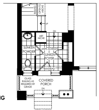
PARTIAL GROUND FLOOR PLAN ELEV. 'A' W/ SUNKEN FOYER CONDITION
