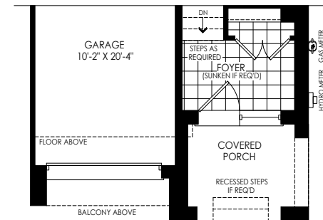
PARTIAL GROUND FLOOR PLAN ELEV 'M4'
