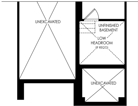
PARTIAL BASEMENT PLAN ELEV 'M1'
