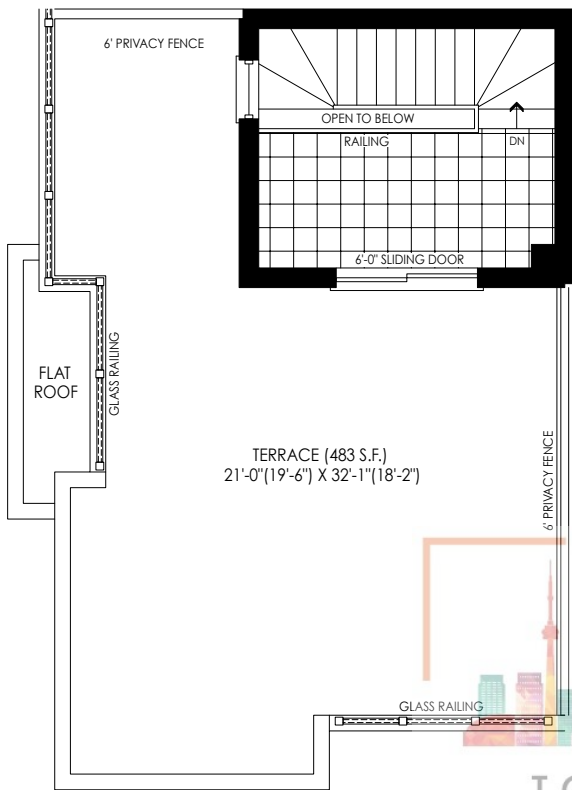
ROOF TERRACE PLAN ELEV. 'M3'
