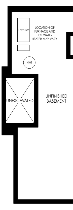
PARTIAL BASEMENT PLAN ELEV. 'FC5'
