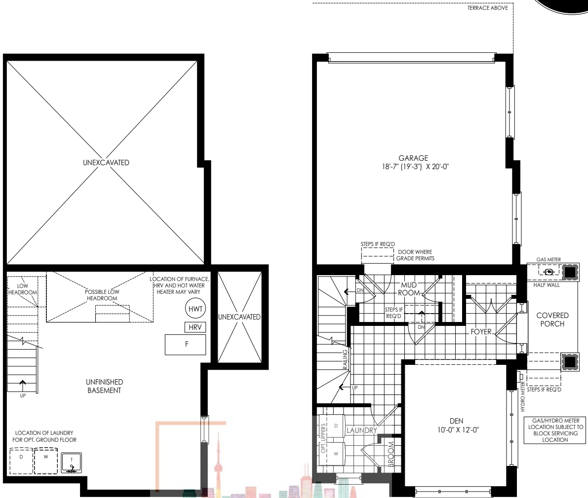
BASEMENT PLAN ELEV. 'F1', 'FC1', 'WC1' & 'M1'
