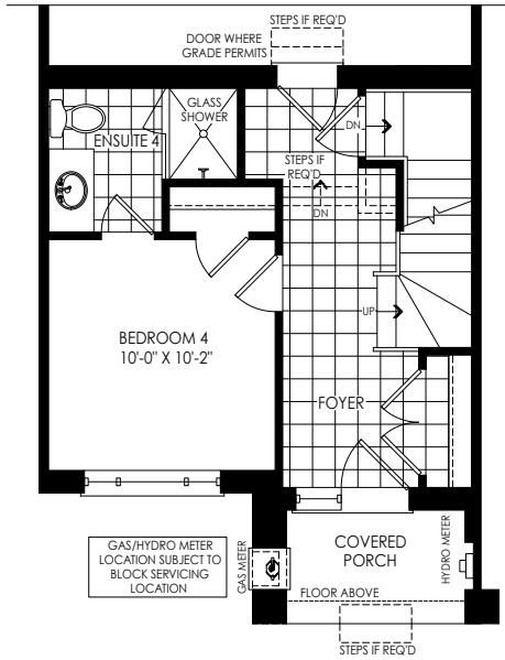
PARTIAL OPT. GROUND FLOOR PLAN W/ 4 BEDROOMS ELEV. 'WC1'
