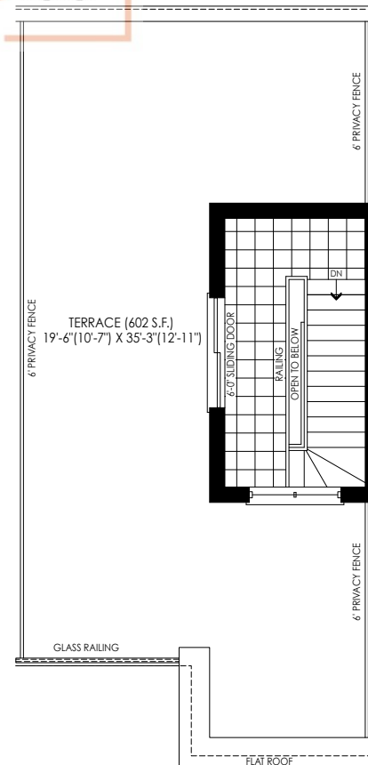
ROOF TERRACE PLAN ELEV. 'WC1'
