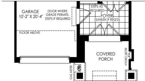
PARTIAL GROUND FLOOR PLAN ELEV 'T2' & 'T4'
