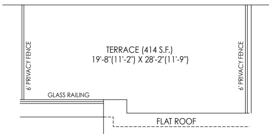
PARTIAL ROOF TERRACE PLAN ELEV. 'WC2'
