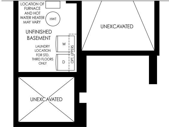
PARTIAL BASEMENT PLAN ELEV. 'M1'
