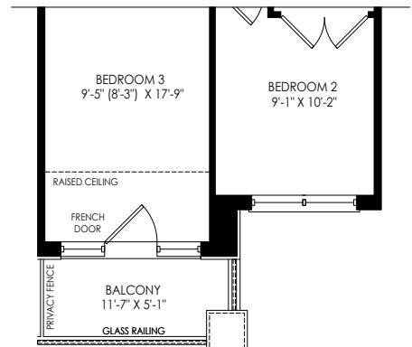
PARTIAL SECOND FLOOR PLAN ELEV 'WC1'
