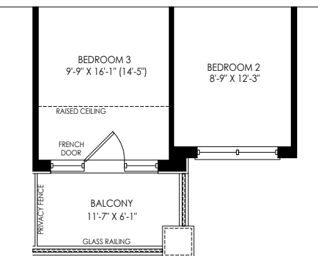
PARTIAL SECOND FLOOR PLAN ELEV 'WC2'
