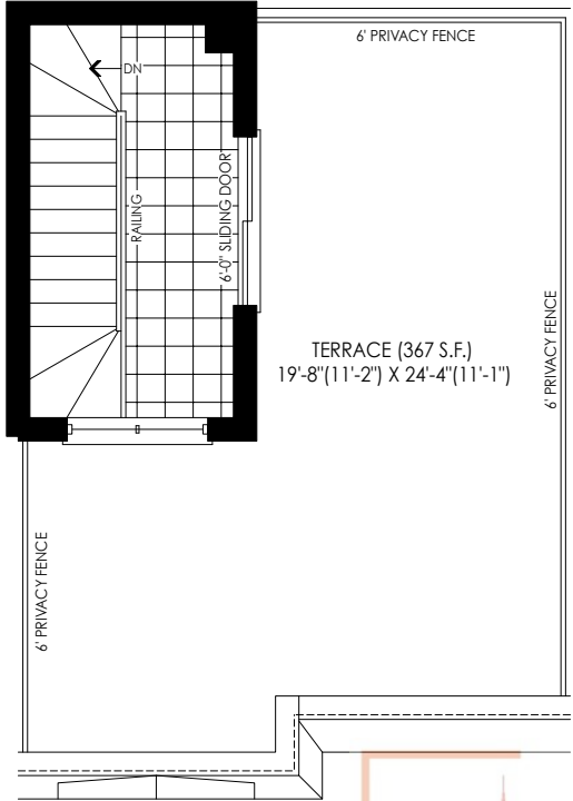
ROOF TERRACE PLAN ELEV. 'FC1'
