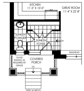
PARTIAL GROUND FLOOR PLAN ELEV. 'A' W/ SUNKEN FOYER CONDITION
