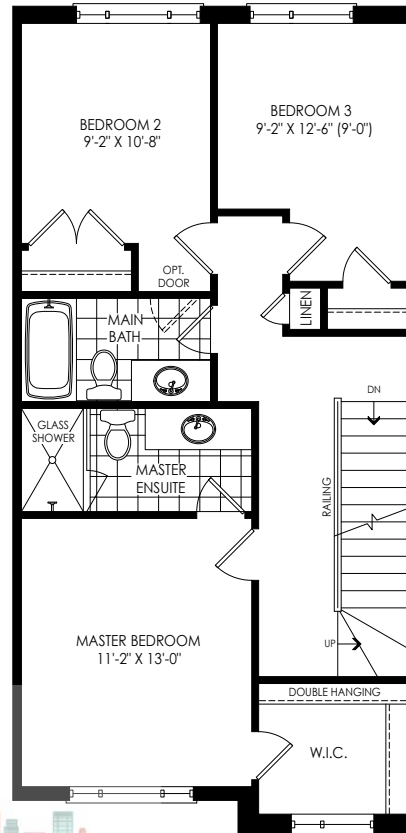
THIRD FLOOR PLAN ELEV. 'M2'
