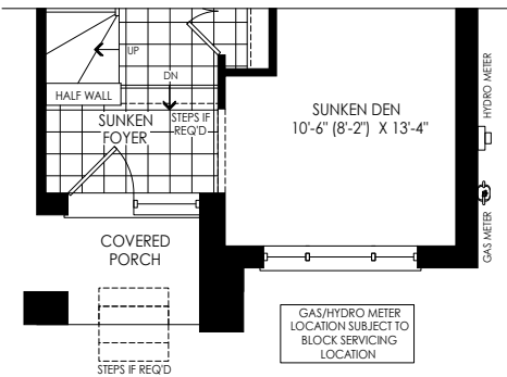
PARTIAL GROUND FLOOR PLAN ELEV. 'M1' W/ SUNKEN FOYER CONDITION
