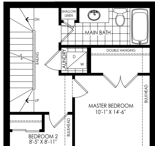
PARTIAL OPT. THIRD FLOOR PLAN W/ LAUNDRY ELEV. 'FC1'
