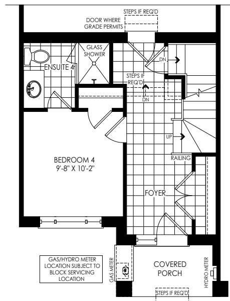
PARTIAL OPT. GROUND FLOOR PLAN W/ 4 BEDROOMS ELEV. 'WC1' & 'M1'
