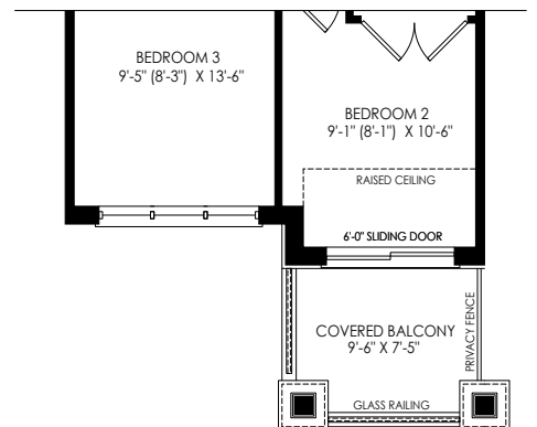
PARTIAL SECOND FLOOR PLAN ELEV 'WC4'
