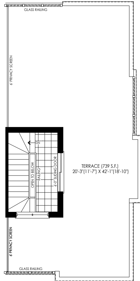
ROOF TERRACE PLAN ELEV. 'M1'
