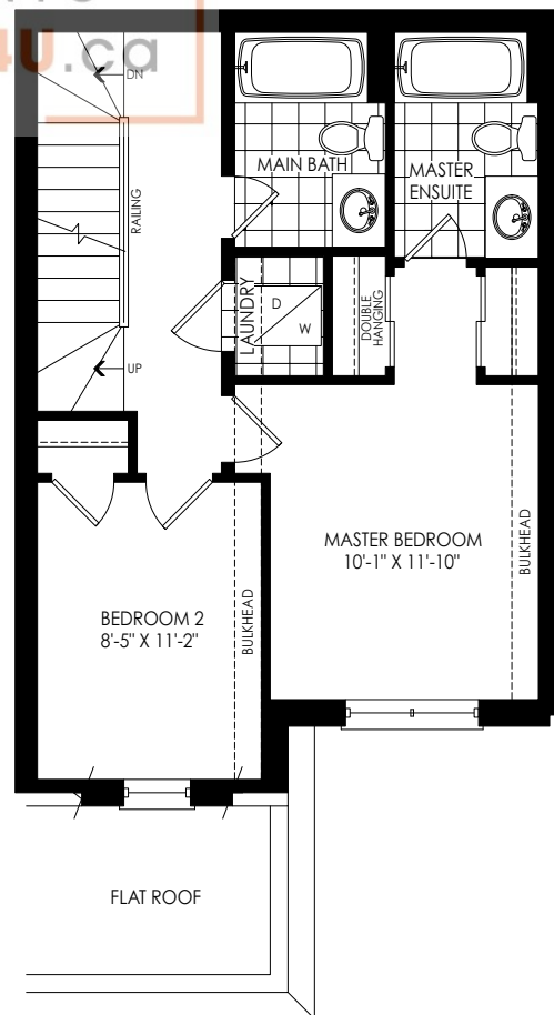
THIRD FLOOR PLAN ELEV. 'FC1'
