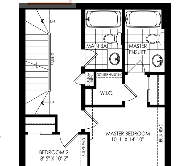
PARTIAL OPT. THIRD FLOOR PLAN W/ WALK-IN CLOSET ELEV. 'WC1' & 'WC2'
