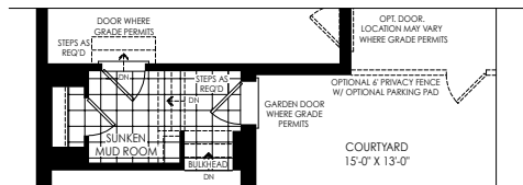
PARTIAL GROUND FLOOR PLAN ELEV. 'A', 'B' & 'D' W/ SUNKEN MUD ROOM CONDITION
