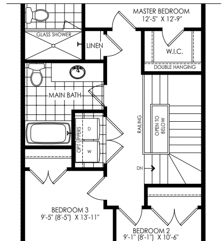
PARTIAL OPT. SECOND FLOOR PLAN W/ LAUNDRY ELEV 'M2' & 'M3'
