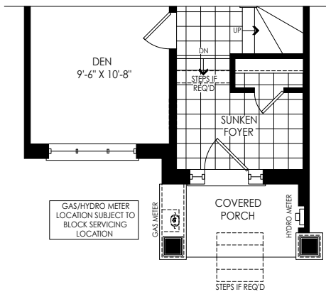
PARTIAL GROUND FLOOR PLAN ELEV. 'F1' & 'FC1' W/ SUNKEN FOYER CONDITION
