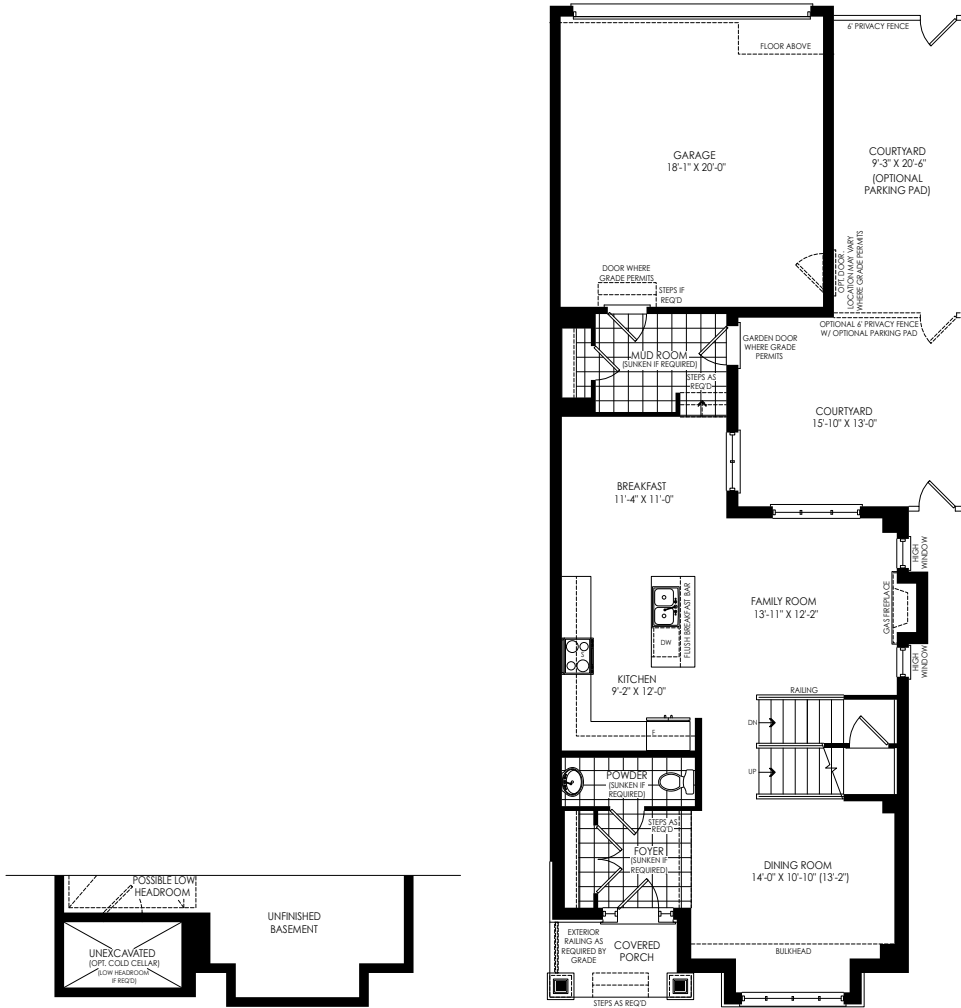
PARTIAL BASEMENT PLAN ELEV. 'D'
