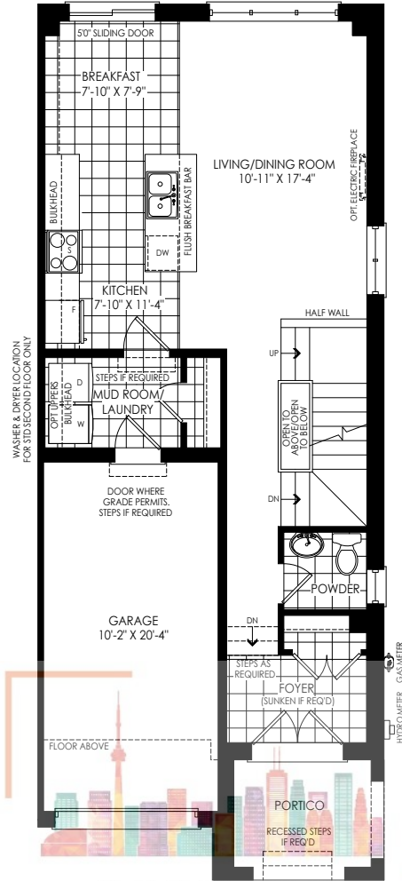
GROUND FLOOR PLAN ELEV 'T3'
