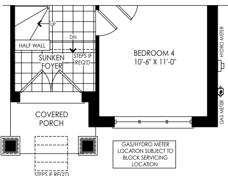
PARTIAL OPT. GROUND FLOOR PLAN W/ 4 BEDROOMS ELEV. 'F1' W/ SUNKEN FOYER CONDITION
