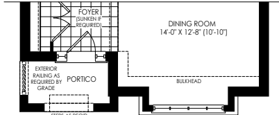
PARTIAL GROUND FLOOR PLAN ELEV. 'E'
