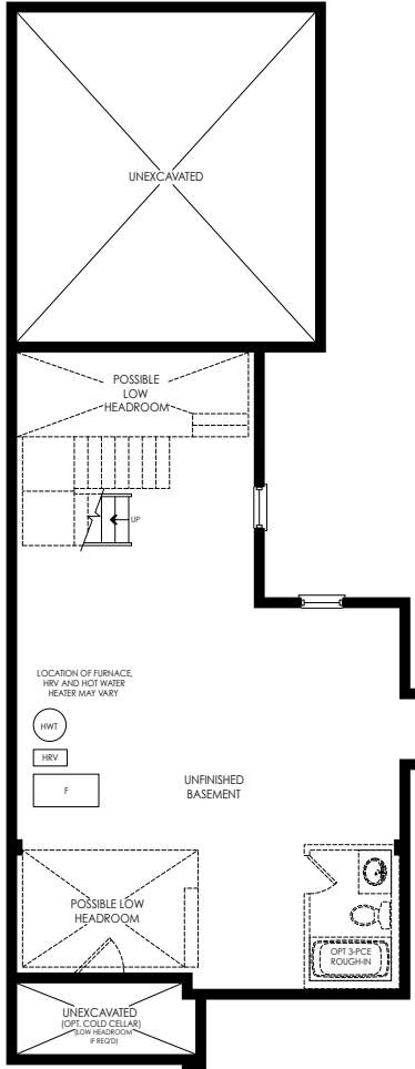
BASEMENT PLAN ELEV. 'A'
