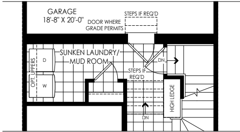
PARTIAL GROUND FLOOR PLAN ELEV. 'F1', 'FC1', 'WC1' & 'M1' W/ SUNKEN MUD ROOM CONDITION
