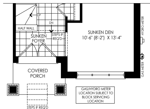
PARTIAL GROUND FLOOR PLAN ELEV. 'FC1' W/ SUNKEN FOYER CONDITION
