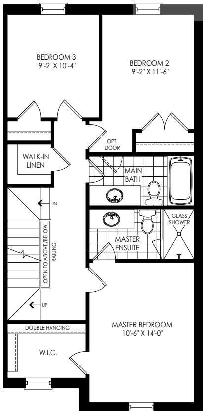
THIRD FLOOR PLAN ELEV. 'FC1'
