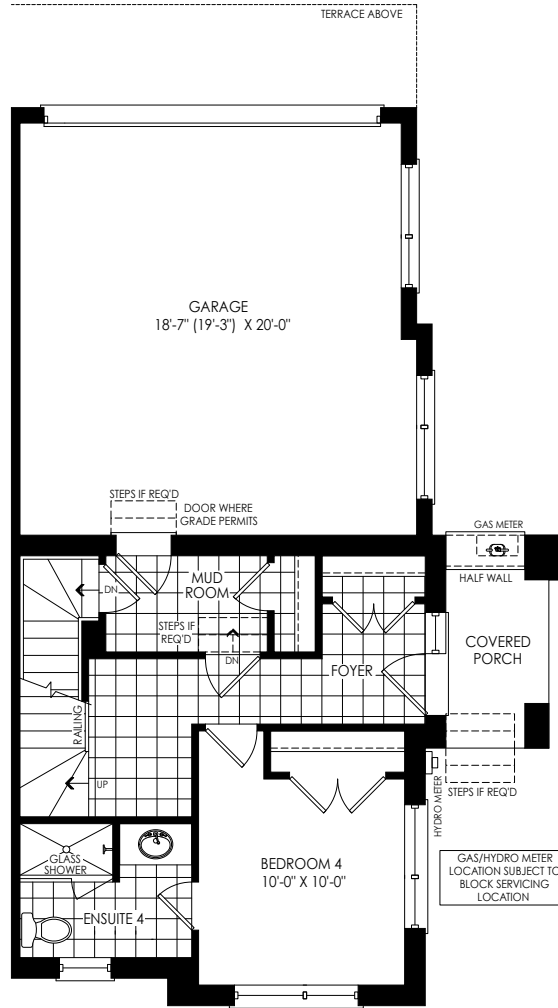
OPT. GROUND FLOOR PLAN W/ 4 BEDROOMS ELEV. 'M1'
