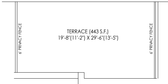
PARTIAL ROOF TERRACE PLAN ELEV. 'M1'
