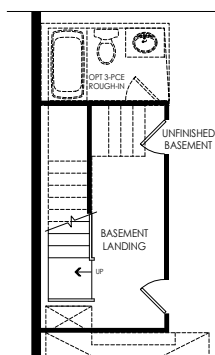
PARTIAL OPT. BASEMENT PLAN W/ FINISHED LANDING ELEV. 'A', 'B' & 'D'
