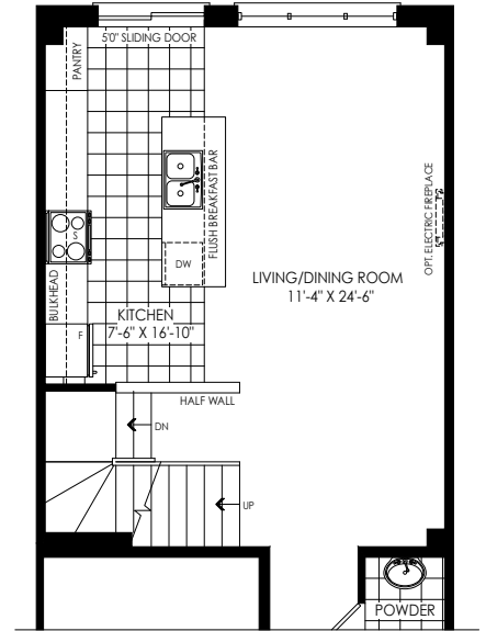
PARTIAL OPT. GROUND FLOOR PLAN W/ ALT. KITCHEN LAYOUT ELEV 'T1', 'T2', 'T4', 'WC1', 'WC2', 'WC3', 'WC4', 'M1', 'M2' & 'M3'
