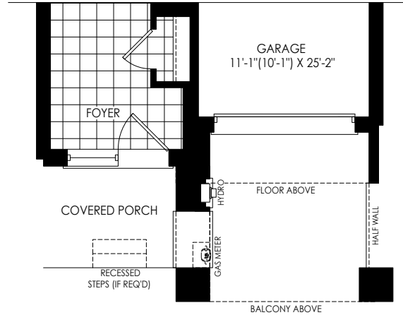
PARTIAL GROUND FLOOR PLAN ELEV. 'WC1' & 'WC2'
