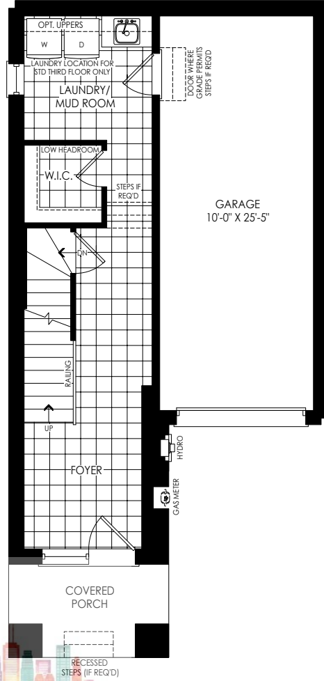
GROUND FLOOR PLAN ELEV. 'WC3'
