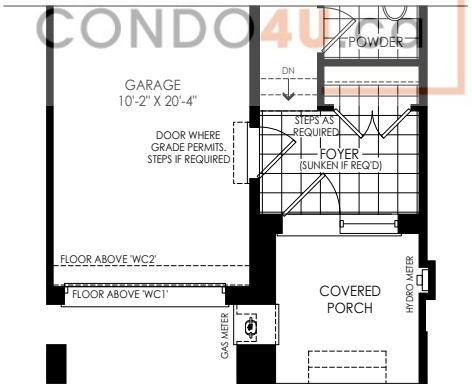
PARTIAL GROUND FLOOR PLAN ELEV 'WC1' & 'WC2'
