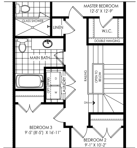
PARTIAL OPT. SECOND FLOOR PLAN W/ LAUNDRY ELEV 'WC1'
