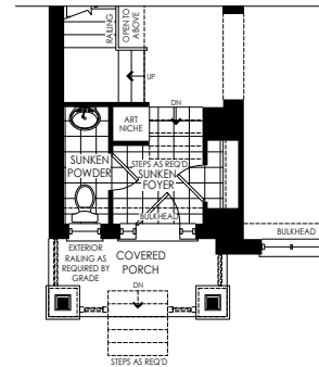
PARTIAL GROUND FLOOR PLAN ELEV. 'E' W/ SUNKEN FOYER CONDITION
