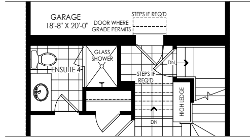
PARTIAL OPT. GROUND FLOOR PLAN W/ 4 BEDROOMS ELEV. 'F1', 'FC1', 'WC1' & 'M1' W/ SUNKEN MUD ROOM CONDITION
