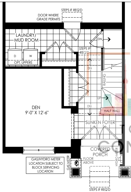
PARTIAL GROUND FLOOR PLAN ELEV. 'F1' & 'FC1' W/ SUNKEN FOYER CONDITION
