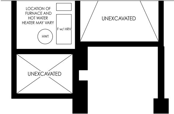
PARTIAL BASEMENT PLAN ELEV. 'WC1' & 'WC2'
