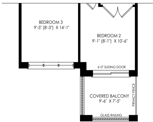
PARTIAL SECOND FLOOR PLAN ELEV 'M3'
