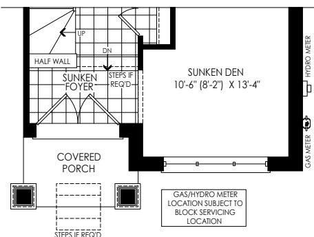
PARTIAL GROUND FLOOR PLAN ELEV. 'F1' W/ SUNKEN FOYER CONDITION
