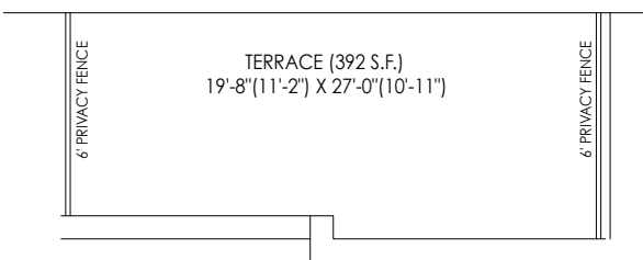
PARTIAL ROOF TERRACE PLAN ELEV. 'M1'
