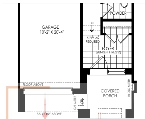
PARTIAL GROUND FLOOR PLAN ELEV 'M1'
