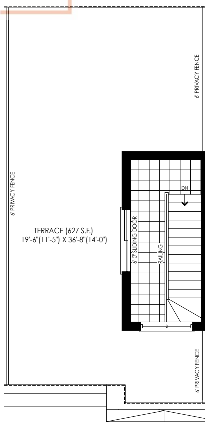
ROOF TERRACE PLAN ELEV. 'FC1'
