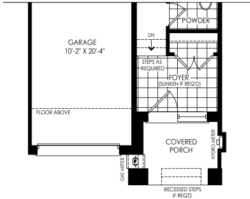
PARTIAL GROUND FLOOR PLAN ELEV 'M2'
