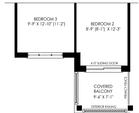
PARTIAL SECOND FLOOR PLAN ELEV 'T4'
