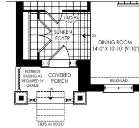
PARTIAL GROUND FLOOR PLAN ELEV. 'C' W/ SUNKEN FOYER CONDITION
