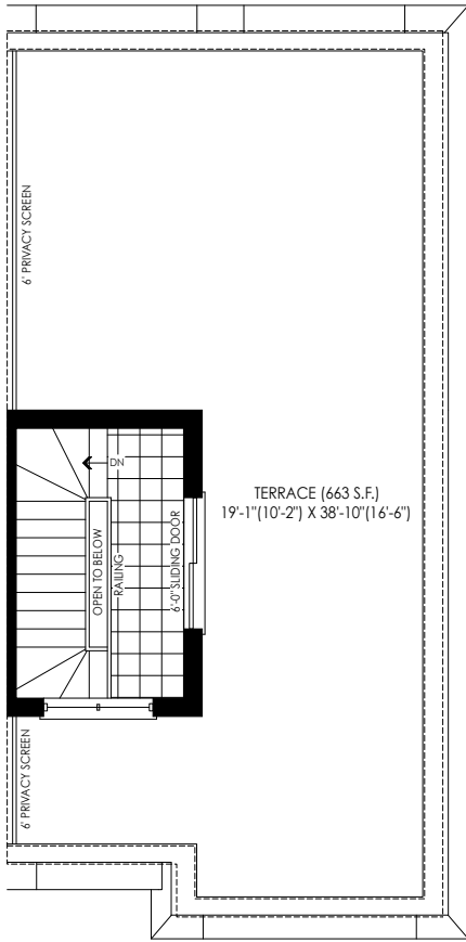
ROOF TERRACE PLAN ELEV. 'F1'
