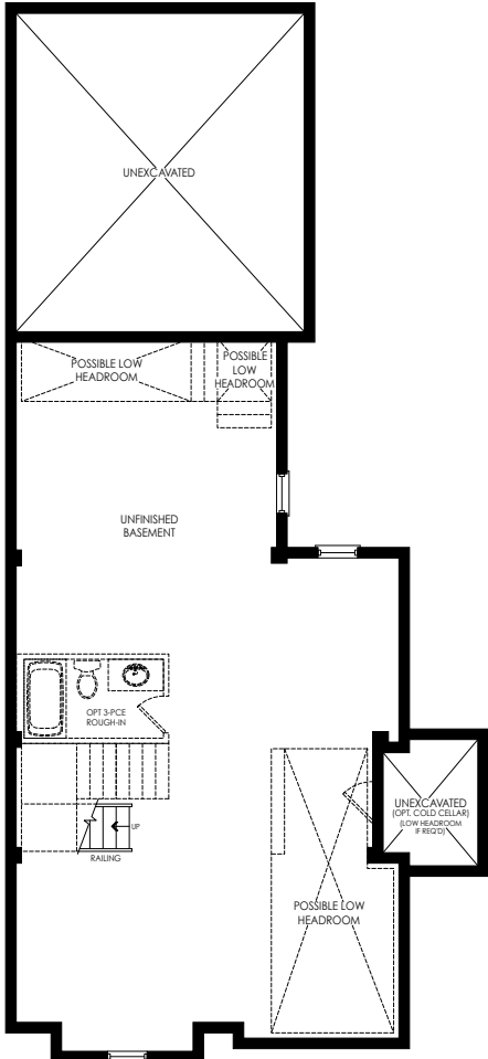
BASEMENT PLAN ELEV. 'D'
