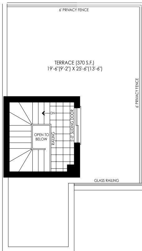
ROOF TERRACE PLAN ELEV. 'M2'
