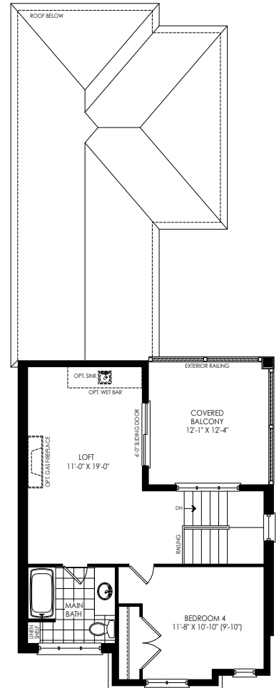
OPT. LOFT PLAN W/ GUEST SUITE ELEV. 'C'
