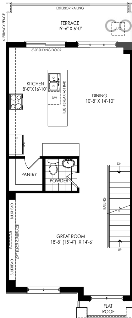
SECOND FLOOR PLAN ELEV. 'F1'
