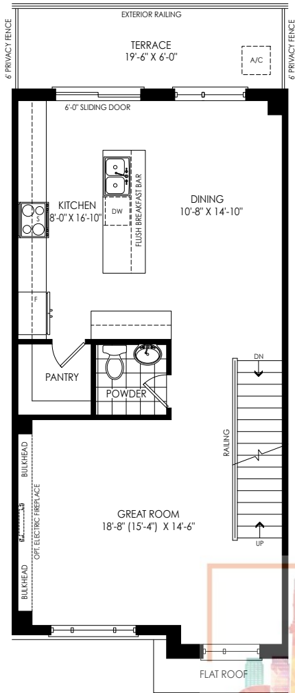
SECOND FLOOR PLAN ELEV. 'M2'
