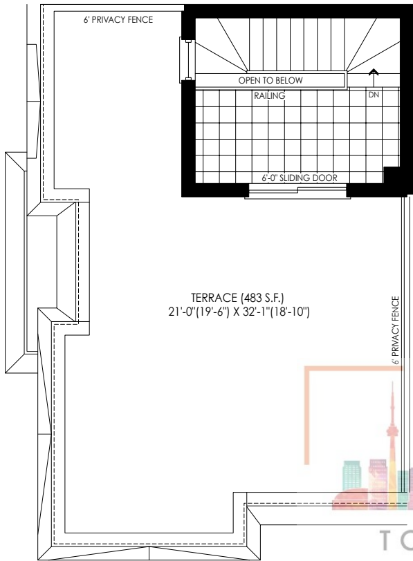
ROOF TERRACE PLAN ELEV. 'FC4'
