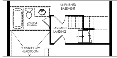
PARTIAL OPT. BASEMENT PLAN W/ FINISHED LANDING ELEV. 'A', 'C' & 'D'
