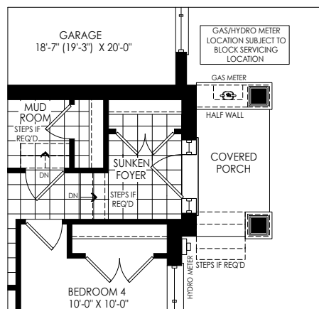
PARTIAL OPT. GROUND FLOOR PLAN W/ 4 BEDROOMS ELEV. 'F1' & 'FC1' W/ SUNKEN FOYER CONDITION
