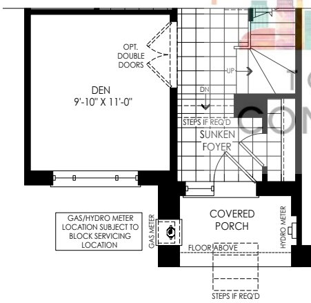
PARTIAL GROUND FLOOR PLAN ELEV. 'WC1' W/ SUNKEN FOYER CONDITION
