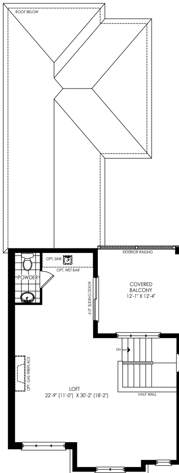
LOFT PLAN ELEV. 'C'
