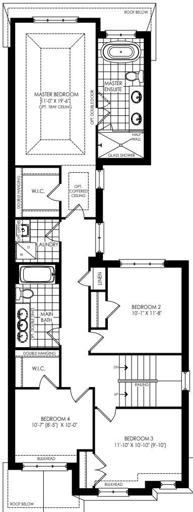
SECOND FLOOR PLAN ELEV. 'C'
