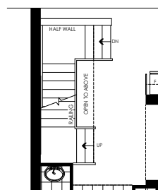
PARTIAL GROUND FLOOR PLAN FOR OPT. FINISHED BASEMENT LANDING ELEV. 'A', 'B' & 'D'
