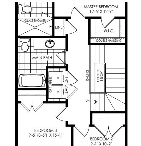
PARTIAL OPT. SECOND FLOOR PLAN W/ LAUNDRY ELEV 'WC2'
