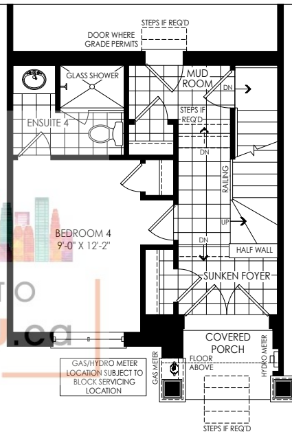
PARTIAL OPT. GROUND FLOOR PLAN W/ 4 BEDROOMS ELEV. 'F1' & 'FC1' W/ SUNKEN FOYER CONDITION
