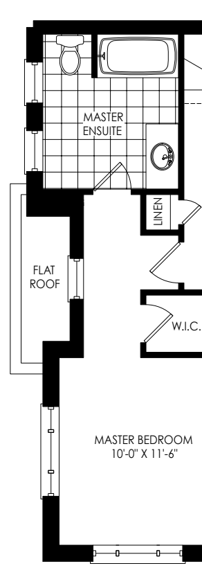
PARTIAL OPT. THIRD FLOOR PLAN ELEV. 'M4'
