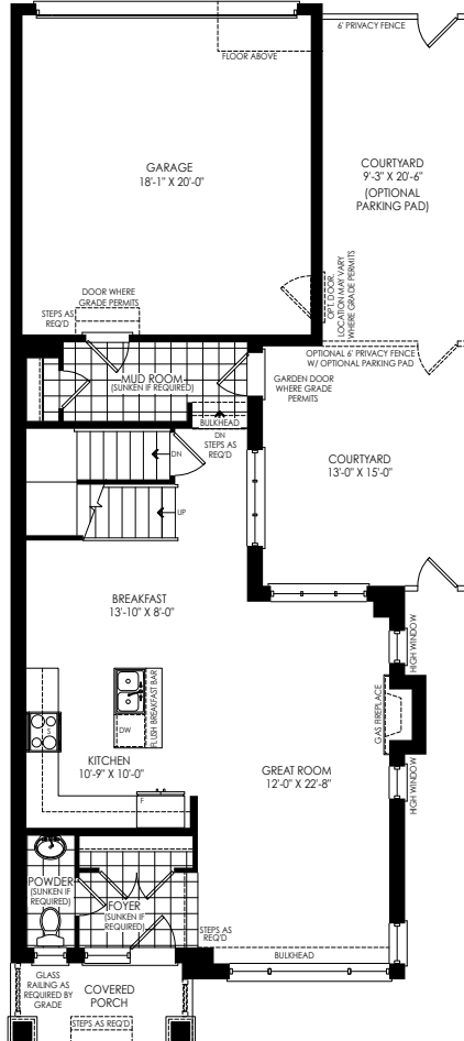
GROUND FLOOR PLAN ELEV. 'A'
