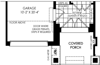
PARTIAL GROUND FLOOR PLAN ELEV 'T2' & 'T4'
