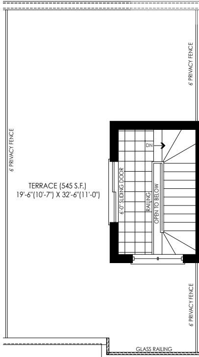
ROOF TERRACE PLAN ELEV. 'M1'
