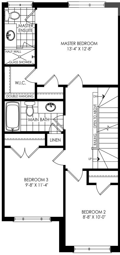
THIRD FLOOR PLAN ELEV. 'M1'
