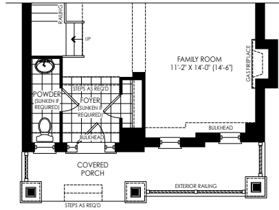
PARTIAL GROUND FLOOR PLAN ELEV. 'B'
