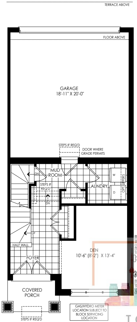
GROUND FLOOR PLAN ELEV. 'FC1'
