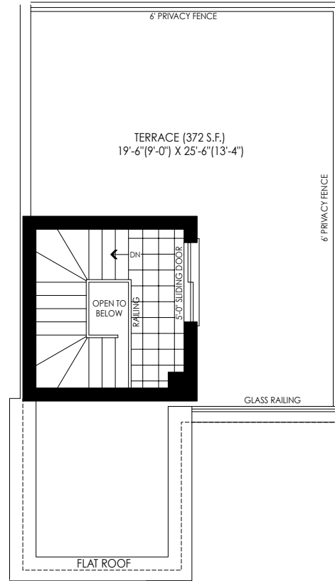
ROOF TERRACE PLAN ELEV. 'WC3'
