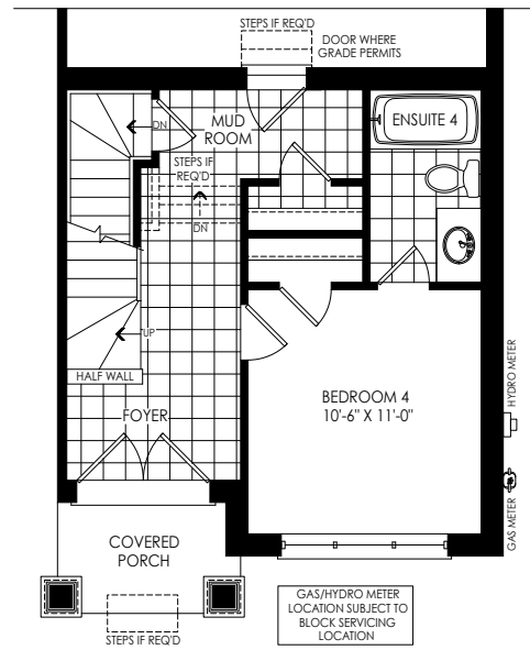
PARTIAL OPT. GROUND FLOOR PLAN W/ 4 BEDROOMS ELEV. 'FC1'
