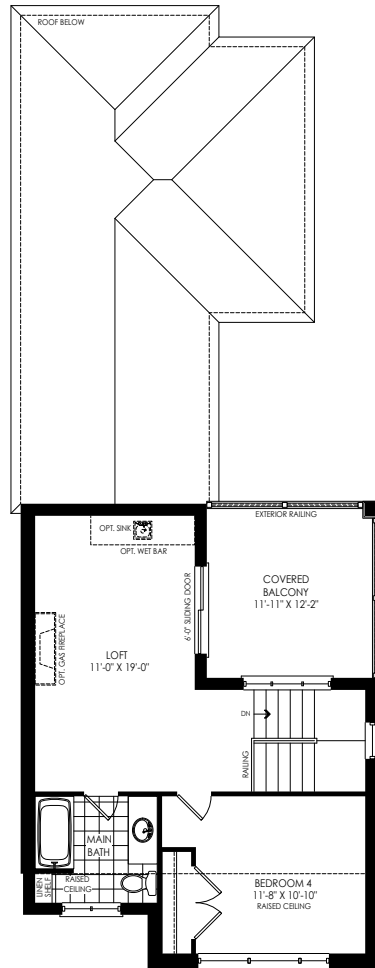
OPT. LOFT PLAN W/ GUEST SUITE ELEV. 'A'
