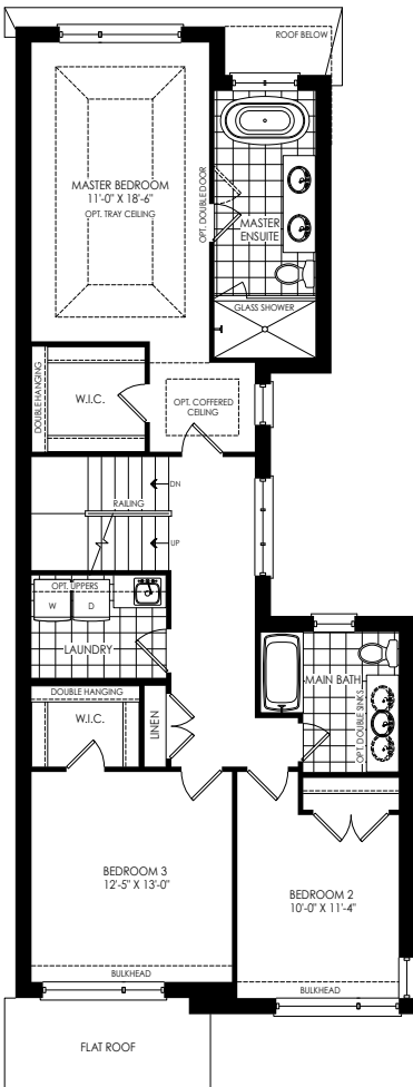
SECOND FLOOR PLAN ELEV. 'A'
