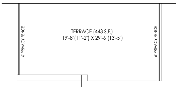
PARTIAL ROOF TERRACE PLAN ELEV. 'M1'
