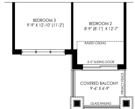
PARTIAL SECOND FLOOR PLAN ELEV 'WC4'
