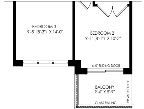
PARTIAL SECOND FLOOR PLAN ELEV 'M2'
