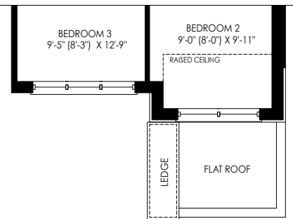
PARTIAL SECOND FLOOR PLAN ELEV 'WC5'
