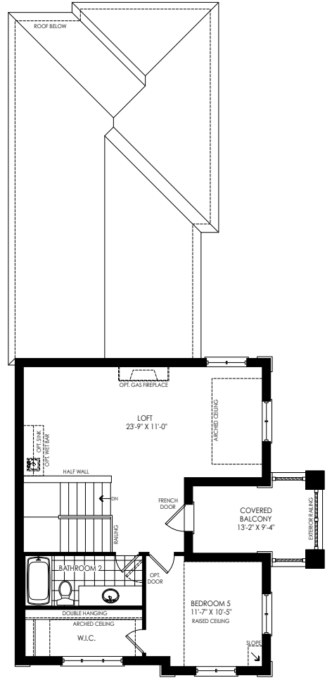
OPT. LOFT PLAN W/ GUEST SUITE ELEV. 'D'
