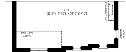
PARTIAL LOFT PLAN ELEV. 'B'
