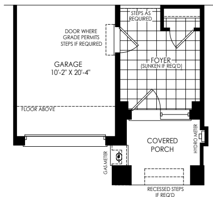
PARTIAL GROUND FLOOR PLAN ELEV 'M3'
