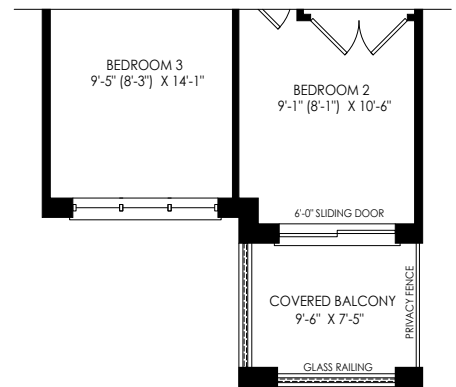
PARTIAL SECOND FLOOR PLAN ELEV 'M3'
