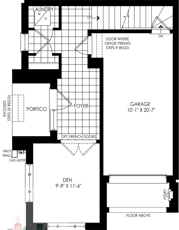
GROUND FLOOR PLAN ELEV. 'WC4'
