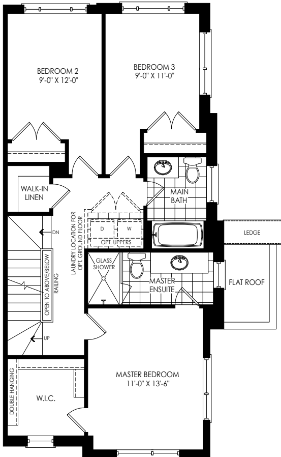
THIRD FLOOR PLAN ELEV. 'M1'
