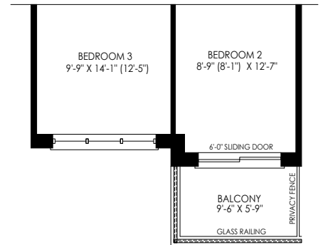
PARTIAL SECOND FLOOR PLAN ELEV 'M2'
