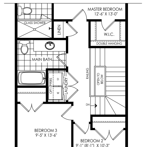
PARTIAL OPT. SECOND FLOOR PLAN W/ LAUNDRY ELEV 'M2' & 'M3'
