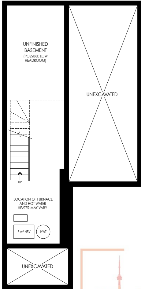
BASEMENT PLAN ELEV. 'WC3' & 'M2'
