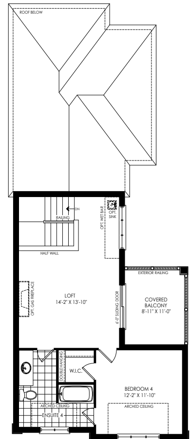
OPT. LOFT PLAN W/ GUEST SUITE ELEV. 'D'
