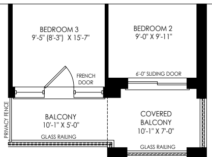
PARTIAL SECOND FLOOR PLAN ELEV 'M4'
