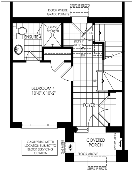
PARTIAL OPT. GROUND FLOOR PLAN W/ 4 BEDROOMS ELEV. 'M1'
