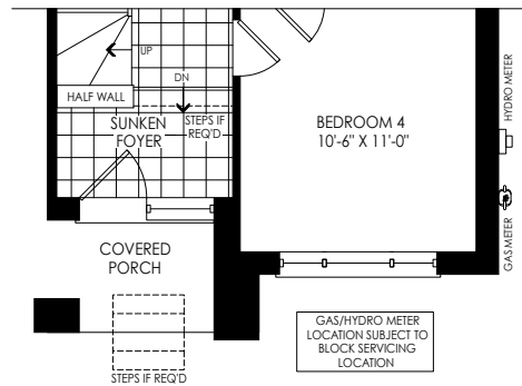
PARTIAL OPT. GROUND FLOOR PLAN W/ 4 BEDROOMS ELEV. 'M1' W/ SUNKEN FOYER CONDITION
