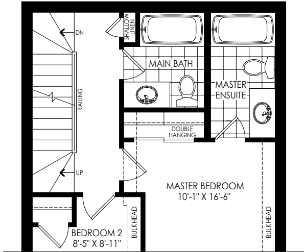
PARTIAL OPT. THIRD FLOOR PLAN W/ MASTER ENSUITE ELEV. 'M1'
