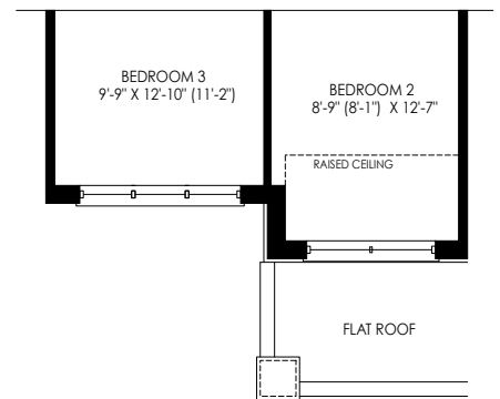
PARTIAL SECOND FLOOR PLAN ELEV 'WC3'
