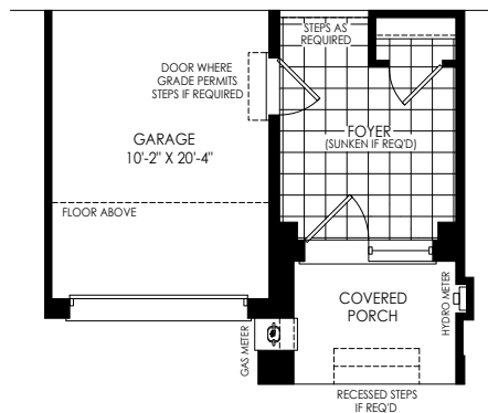
PARTIAL GROUND FLOOR PLAN ELEV 'WC3'
