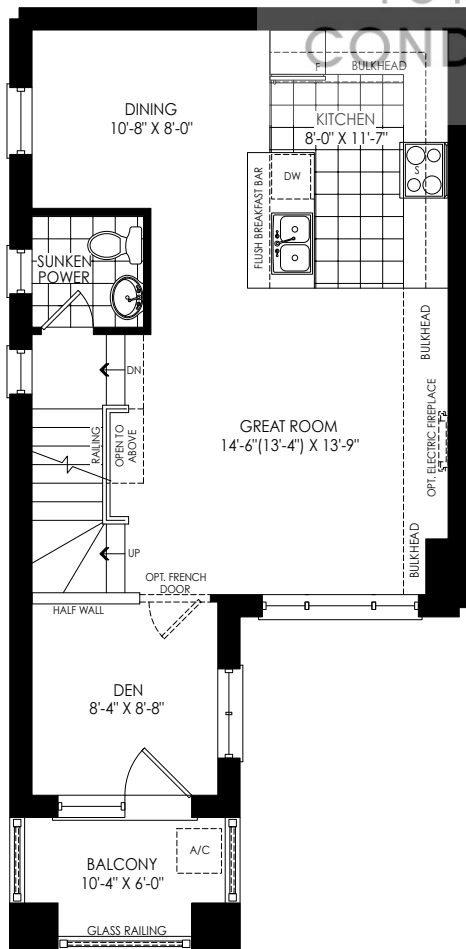
SECOND FLOOR PLAN ELEV. 'WC3'
