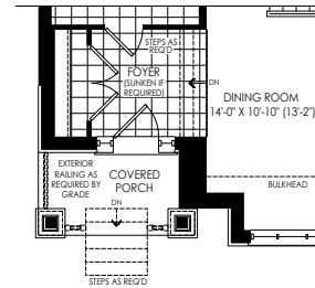
PARTIAL GROUND FLOOR PLAN ELEV. 'D' W/ SUNKEN FOYER CONDITION
