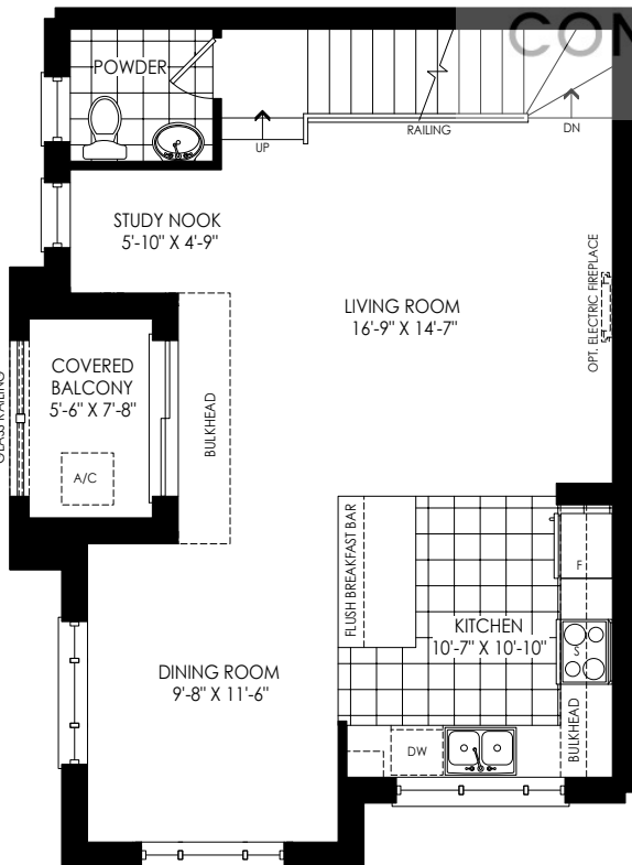
SECOND FLOOR PLAN ELEV. 'M3'
