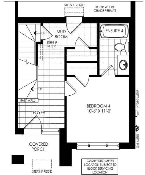
PARTIAL OPT. GROUND FLOOR PLAN W/ 4 BEDROOMS ELEV. 'M1'
