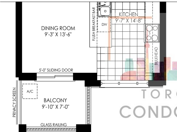
PARTIAL SECOND FLOOR PLAN ELEV. 'M1'
