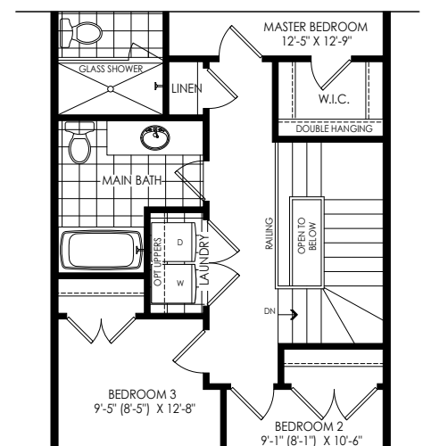
PARTIAL OPT. SECOND FLOOR PLAN W/ LAUNDRY ELEV 'WC3' & 'WC4'
