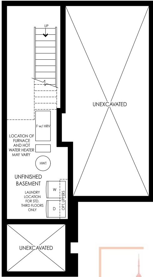
BASEMENT PLAN ELEV. 'FC1' & 'FC2'
