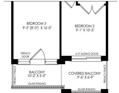
PARTIAL SECOND FLOOR PLAN ELEV 'M1'
