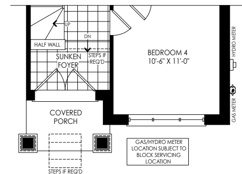
PARTIAL OPT. GROUND FLOOR PLAN W/ 4 BEDROOMS ELEV. 'FC1' W/ SUNKEN FOYER CONDITION
