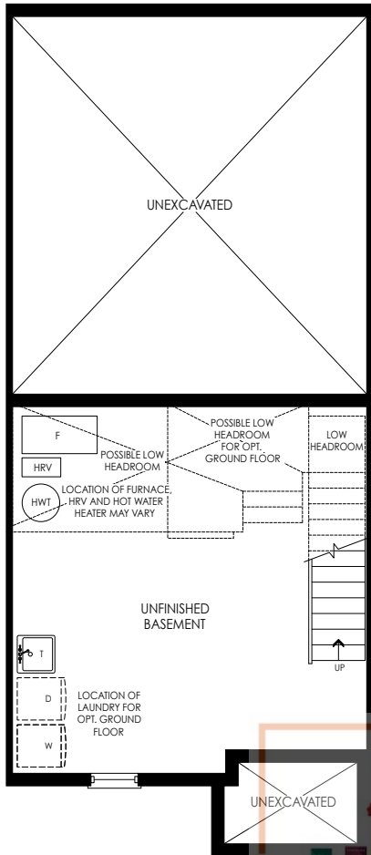
BASEMENT PLAN ELEV. 'F1', 'FC1', 'M1', & 'M2'
