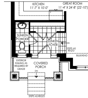
PARTIAL GROUND FLOOR PLAN ELEV. 'D' W/ SUNKEN FOYER CONDITION
