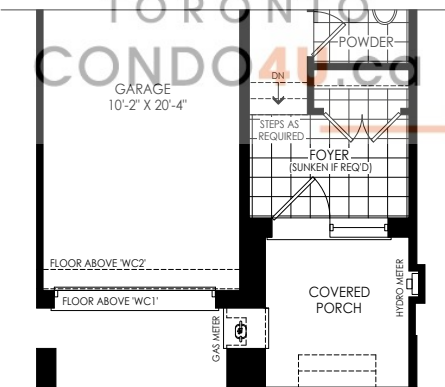
PARTIAL GROUND FLOOR PLAN ELEV 'WC1' & 'WC2'
