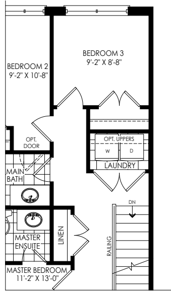
PARTIAL OPT. THIRD FLOOR PLAN W/ LAUNDRY ELEV. 'F1' & 'FC1'
