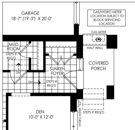
PARTIAL GROUND FLOOR PLAN ELEV. 'M1' W/ SUNKEN FOYER CONDITION
