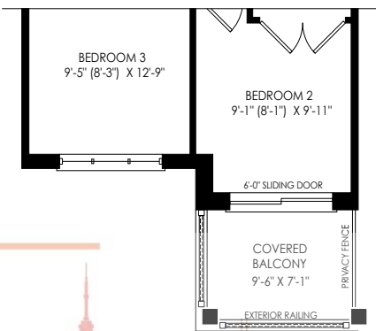
PARTIAL SECOND FLOOR PLAN ELEV 'T4'
