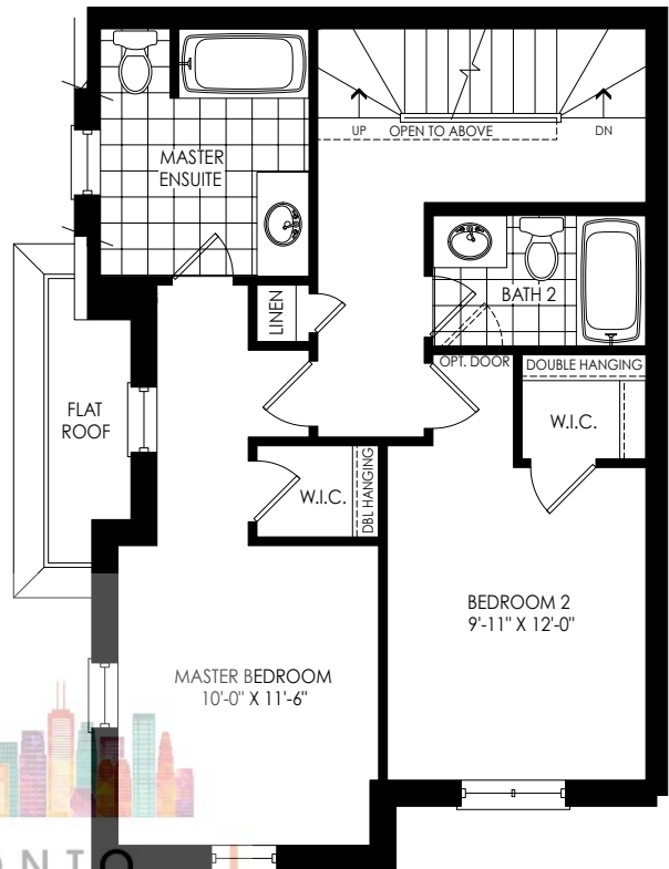
OPT. THIRD FLOOR PLAN W/ 2 BEDROOMS ELEV. 'FC4'
