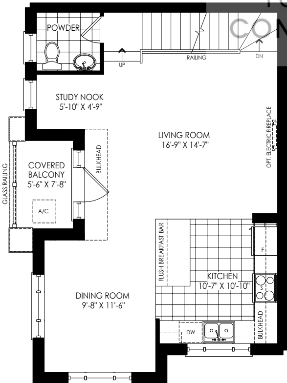
SECOND FLOOR PLAN ELEV. 'WC4'
