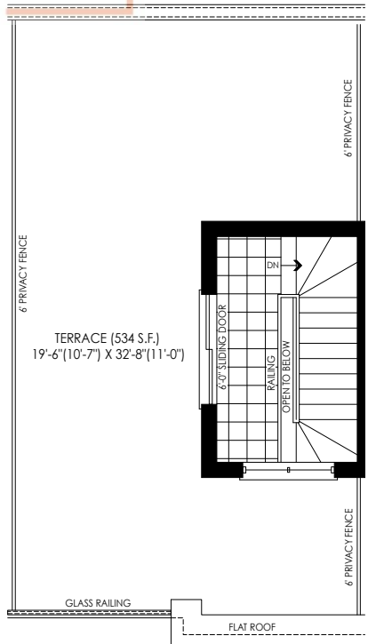
ROOF TERRACE PLAN ELEV. 'WC1'
