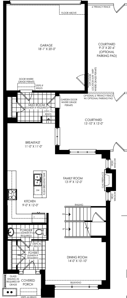
GROUND FLOOR PLAN ELEV. 'A'
