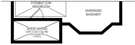
PARTIAL BASEMENT PLAN ELEV. 'D'
