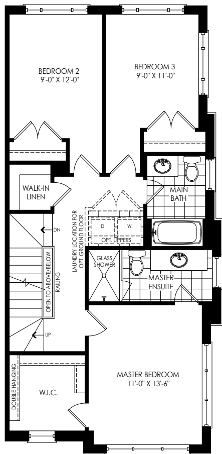
THIRD FLOOR PLAN ELEV. 'WC1'
