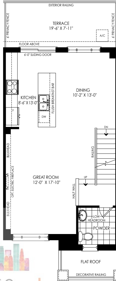
SECOND FLOOR PLAN ELEV. 'WC1'
