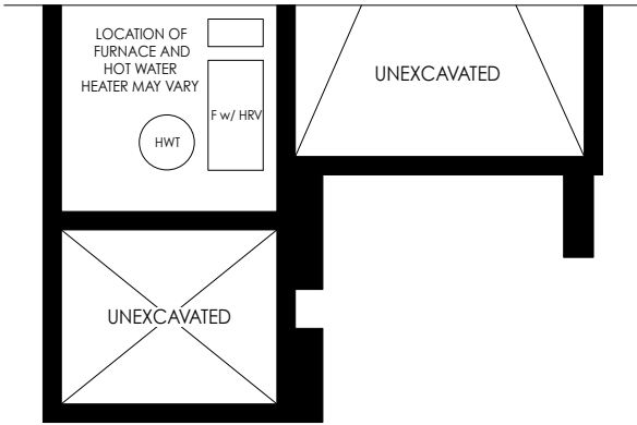
PARTIAL BASEMENT PLAN ELEV. 'M1'
