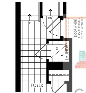
PARTIAL GROUND FLOOR PLAN FOR OPT. THIRD FLOOR ELEV. 'FC1', 'FC2', 'WC1', 'WC2' & 'M1'
