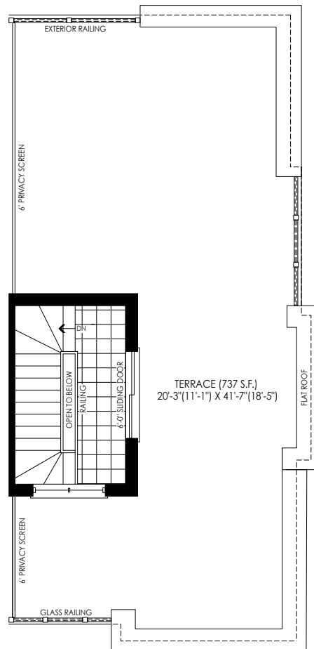
ROOF TERRACE PLAN ELEV. 'WC1'
