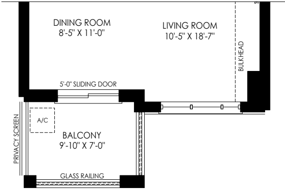
PARTIAL OPT. SECOND FLOOR PLAN W/ ALT. KITCHEN ELEV. 'M1'
