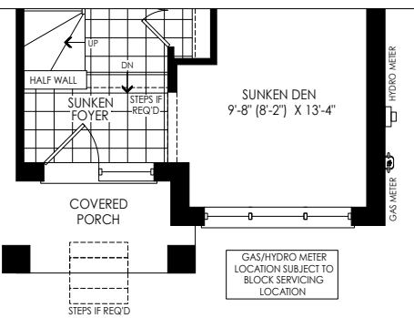
PARTIAL GROUND FLOOR PLAN ELEV. 'WC1' W/ SUNKEN FOYER CONDITION
