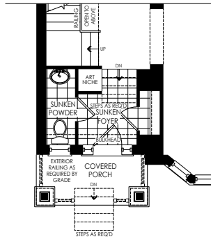
PARTIAL GROUND FLOOR PLAN ELEV. 'B' W/ SUNKEN FOYER CONDITION
