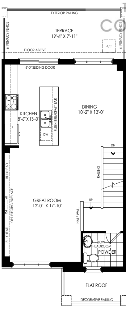
SECOND FLOOR PLAN ELEV. 'F1'
