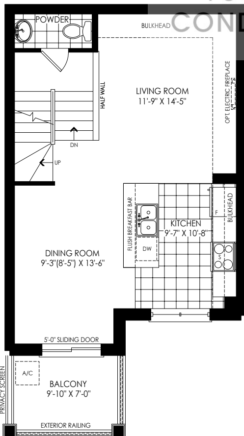
SECOND FLOOR PLAN ELEV. 'FC1' & 'FC2'
