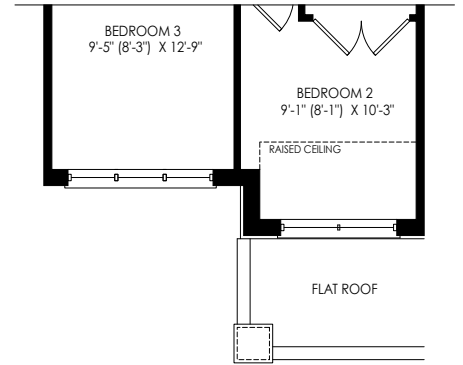
PARTIAL SECOND FLOOR PLAN ELEV 'WC3'
