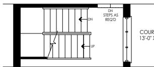
PARTIAL GROUND FLOOR PLAN FOR OPT. FINISHED BASEMENT LANDING ELEV. 'B' & 'A'
