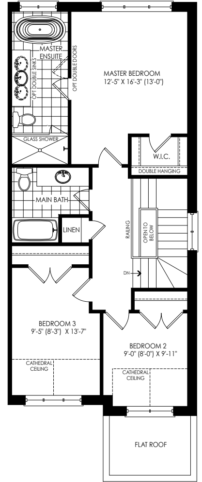
SECOND FLOOR PLAN ELEV 'T3'
