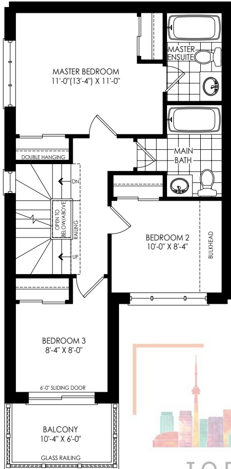
THIRD FLOOR PLAN ELEV. 'M2'
