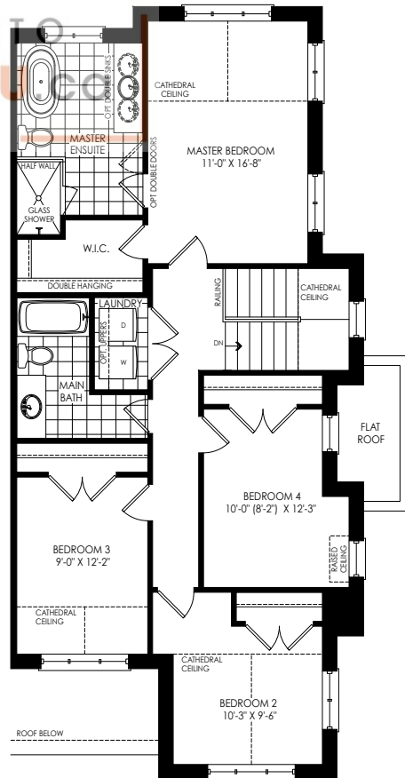
OPT. SECOND FLOOR PLAN W/ 4 BEDROOMS ELEV 'T5'
