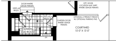
PARTIAL GROUND FLOOR PLAN ELEV. 'E', 'B' & 'A' W/ SUNKEN MUD ROOM CONDITION
