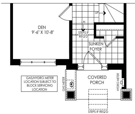
PARTIAL GROUND FLOOR PLAN ELEV. 'F1' & 'FC1' W/ SUNKEN FOYER CONDITION
