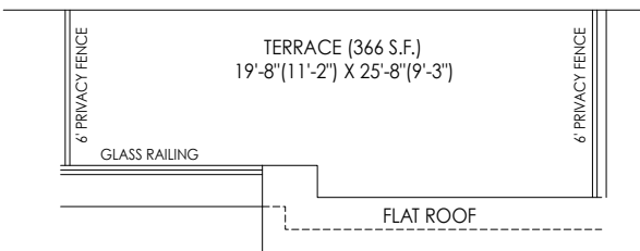
PARTIAL ROOF TERRACE PLAN ELEV. 'WC1'
