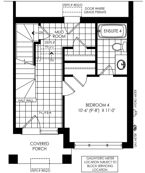
PARTIAL OPT. GROUND FLOOR PLAN W/ 4 BEDROOMS ELEV. 'WC1'
