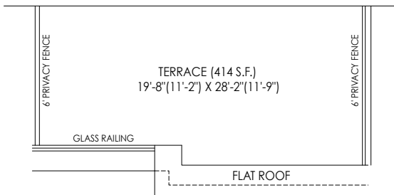
PARTIAL ROOF TERRACE PLAN ELEV. 'WC2'
