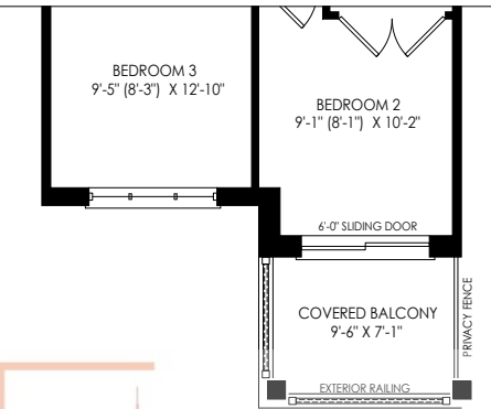
PARTIAL SECOND FLOOR PLAN ELEV 'T4'
