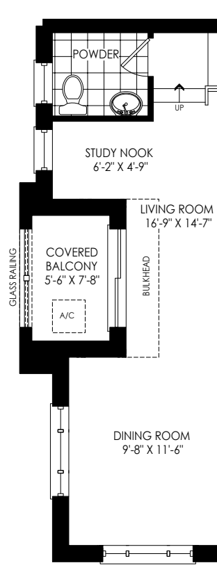
PARTIAL SECOND FLOOR PLAN ELEV. 'M4'
