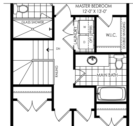
PARTIAL OPT. SECOND FLOOR PLAN W/ LAUNDRY ELEV 'T1', 'T2', 'T4', 'WC1', 'WC2', 'WC3', 'WC4', 'M1', 'M2' & 'M3'
