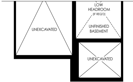
PARTIAL BASEMENT PLAN ELEV 'T2' & 'T4'
