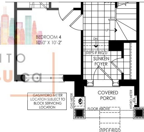
PARTIAL OPT. GROUND FLOOR PLAN W/ 4 BEDROOMS ELEV. 'F1' & 'FC1' W/ SUNKEN FOYER CONDITION
