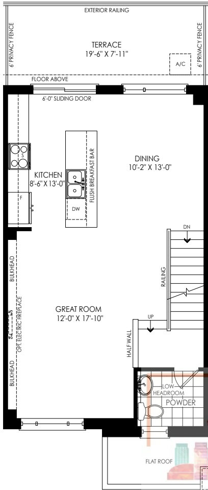
SECOND FLOOR PLAN ELEV. 'M1'
