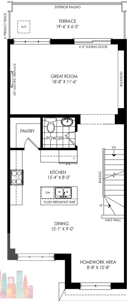
SECOND FLOOR PLAN ELEV. 'FC1'
