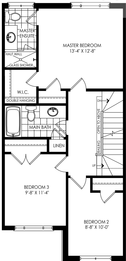
THIRD FLOOR PLAN ELEV. 'WC1'
