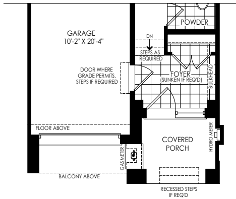
PARTIAL GROUND FLOOR PLAN ELEV 'M1'
