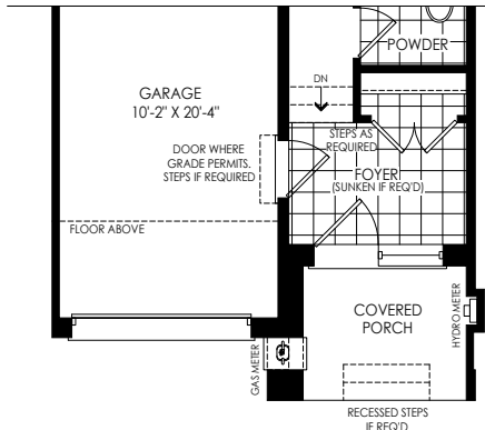
PARTIAL GROUND FLOOR PLAN ELEV 'WC3'
