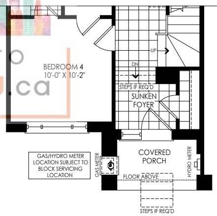
PARTIAL OPT. GROUND FLOOR PLAN W/ 4 BEDROOMS ELEV. 'WC1' W/ SUNKEN FOYER CONDITION
