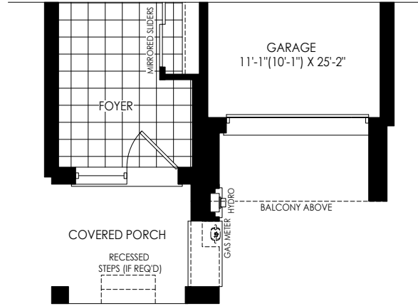
PARTIAL GROUND FLOOR PLAN ELEV. 'M1'
