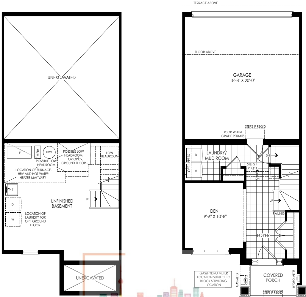
BASEMENT PLAN ELEV. 'F1', 'FC1', 'WC1' & 'M1'
