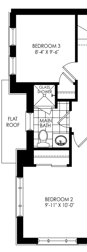
PARTIAL THIRD FLOOR PLAN ELEV. 'WC5'
