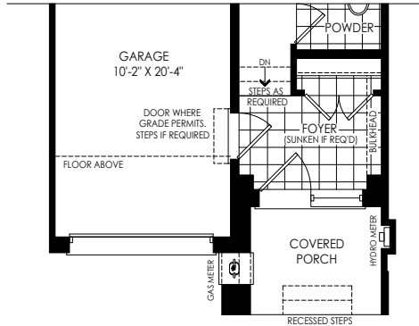
PARTIAL GROUND FLOOR PLAN ELEV 'WC3'
