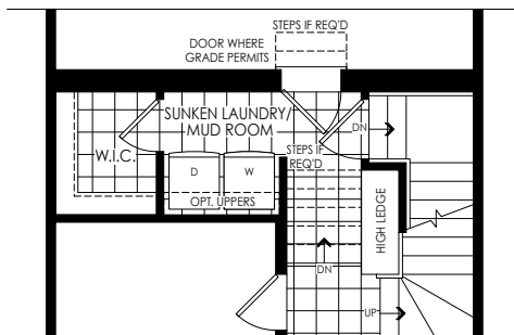
PARTIAL GROUND FLOOR PLAN ELEV. 'F1', 'FC1', 'WC1' & 'M1' W/ SUNKEN MUD ROOM CONDITION
