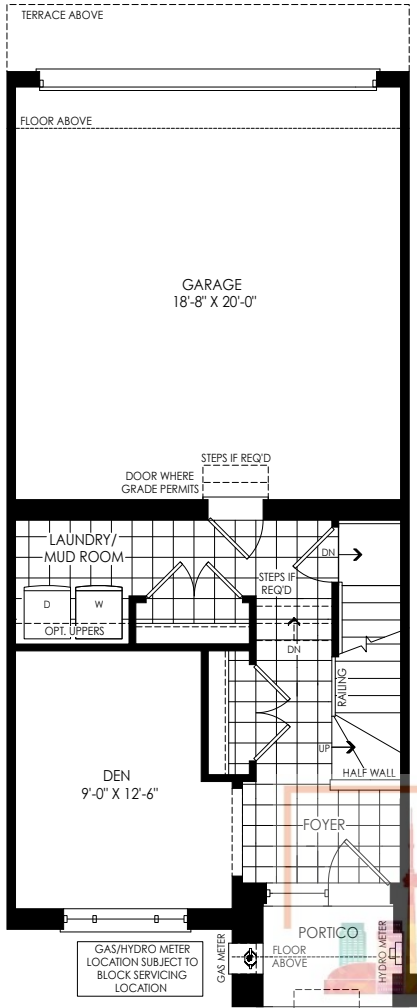
GROUND FLOOR PLAN ELEV. 'M1' & 'M2'
