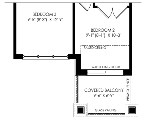
PARTIAL SECOND FLOOR PLAN ELEV 'WC4'
