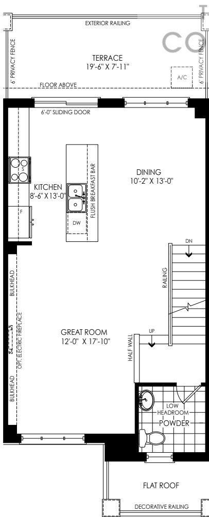
SECOND FLOOR PLAN ELEV. 'F1'
