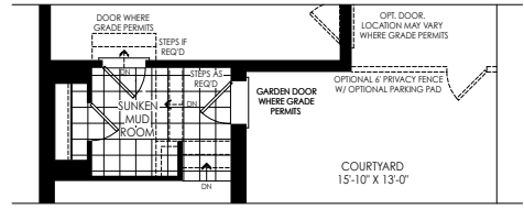
PARTIAL GROUND FLOOR PLAN ELEV. 'A', 'C' & 'D' W/ SUNKEN MUD ROOM CONDITION
