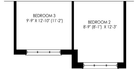
PARTIAL SECOND FLOOR PLAN ELEV 'T2'
