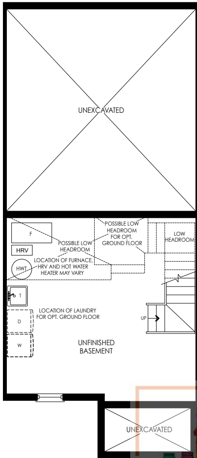
BASEMENT PLAN ELEV. 'F1', 'FC1', 'WC1' & 'M1'
