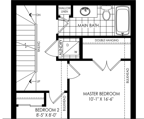
PARTIAL OPT. THIRD FLOOR PLAN W/ LAUNDRY ELEV. 'WC1' & 'WC2'
