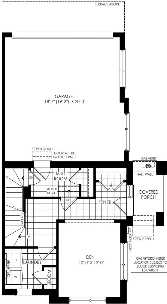
GROUND FLOOR PLAN ELEV. 'M1'
