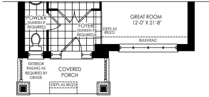
PARTIAL GROUND FLOOR PLAN ELEV. 'B'
