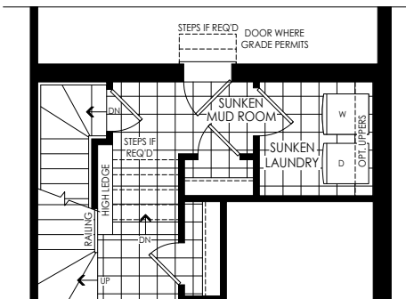
PARTIAL GROUND FLOOR PLAN ELEV. 'F1', 'FC1', 'WC1' & 'M1' W/ SUNKEN MUD ROOM CONDITION
