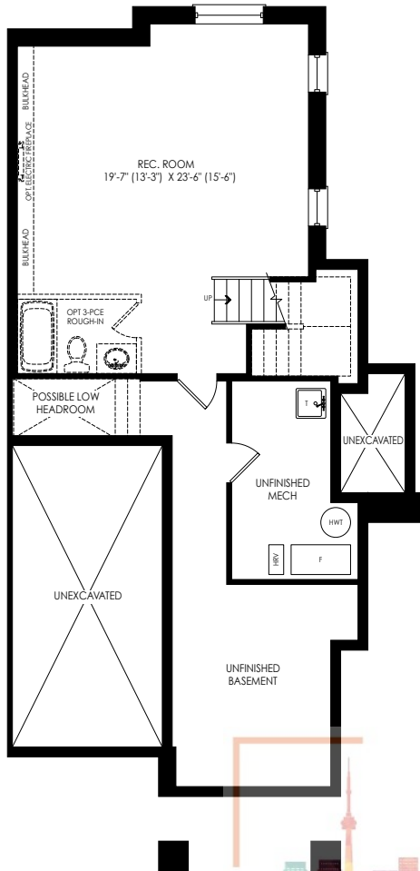
BASEMENT PLAN ELEV 'WC6'
