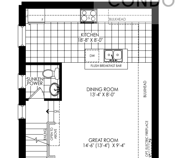
PARTIAL OPT. SECOND FLOOR PLAN W/ ALT. KITCHEN LAYOUT ELEV. 'FC3', 'WC3' & 'M2'
