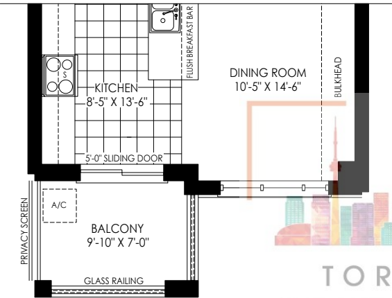
PARTIAL SECOND FLOOR PLAN ELEV. 'M1'
