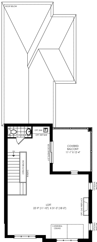
LOFT PLAN ELEV. 'E'
