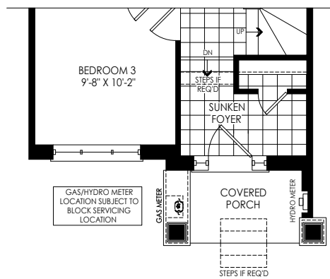
PARTIAL OPT. GROUND FLOOR PLAN W/ 3 BEDROOMS ELEV. 'F1' & 'FC1' W/ SUNKEN FOYER CONDITION
