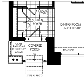
PARTIAL GROUND FLOOR PLAN ELEV. 'A' W/ SUNKEN FOYER CONDITION
