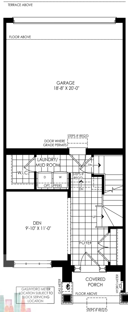
GROUND FLOOR PLAN ELEV. 'F1' & 'FC1'
