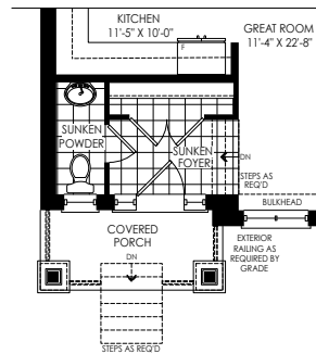
PARTIAL GROUND FLOOR PLAN ELEV. 'B' W/ SUNKEN FOYER CONDITION
