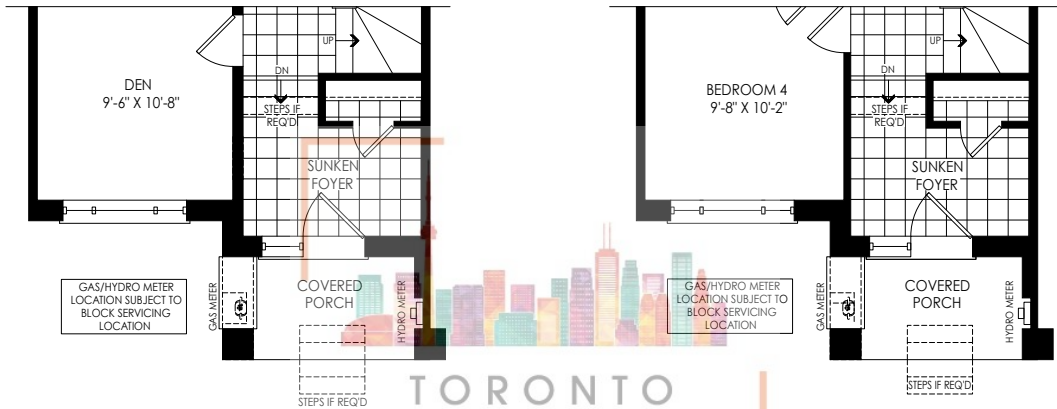
PARTIAL GROUND FLOOR PLAN ELEV. 'WC1' & 'M1' W/ SUNKEN FOYER CONDITION
