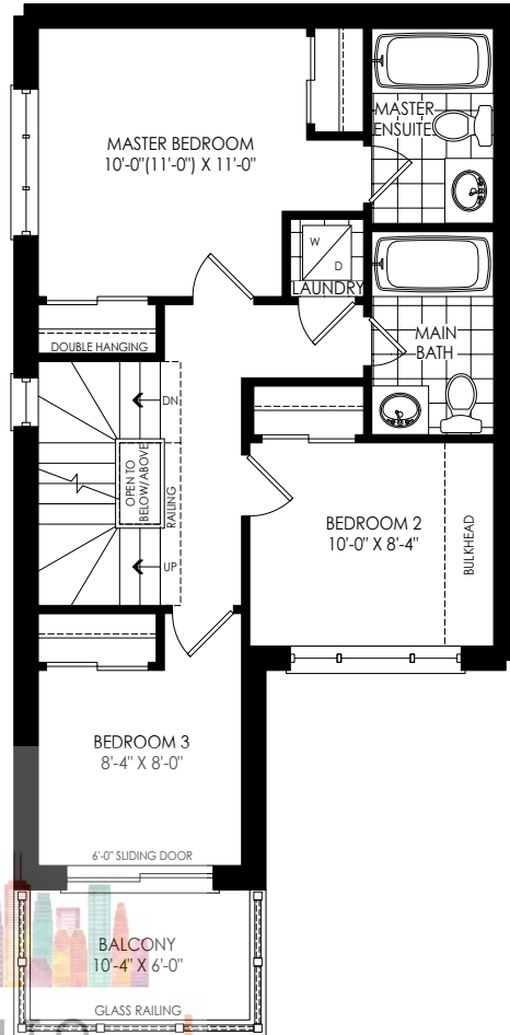
OPT. THIRD FLOOR PLAN W/ LAUNDRY ELEV. 'M2'
