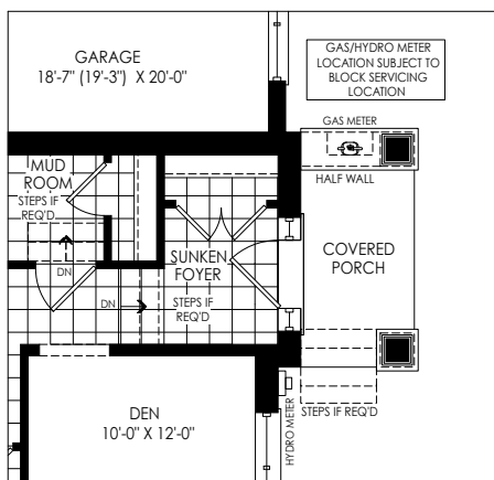
PARTIAL GROUND FLOOR PLAN ELEV. 'F1' & 'FC1' W/ SUNKEN FOYER CONDITION
