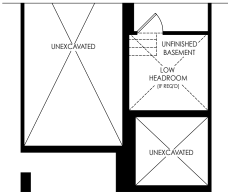
PARTIAL BASEMENT PLAN ELEV 'WC1' & 'WC2'
