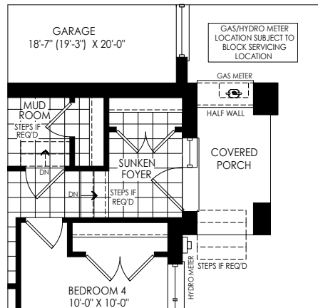
PARTIAL OPT. GROUND FLOOR PLAN W/ 4 BEDROOMS ELEV. 'M1' W/ SUNKEN FOYER CONDITION
