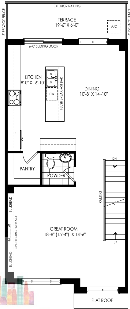
SECOND FLOOR PLAN ELEV. 'M1'
