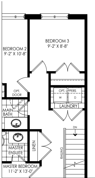
PARTIAL OPT. THIRD FLOOR PLAN W/ LAUNDRY ELEV. 'M1' & 'M2'
