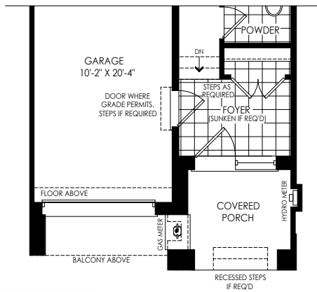
PARTIAL GROUND FLOOR PLAN ELEV 'M1'
