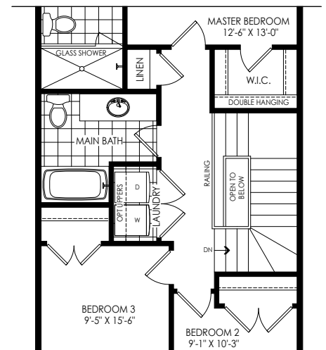
PARTIAL OPT. SECOND FLOOR PLAN W/ LAUNDRY ELEV 'M1'
