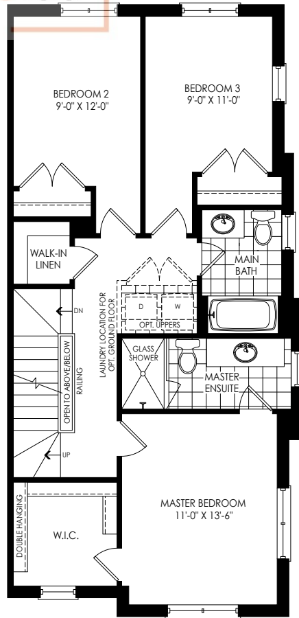
THIRD FLOOR PLAN ELEV. 'F1'
