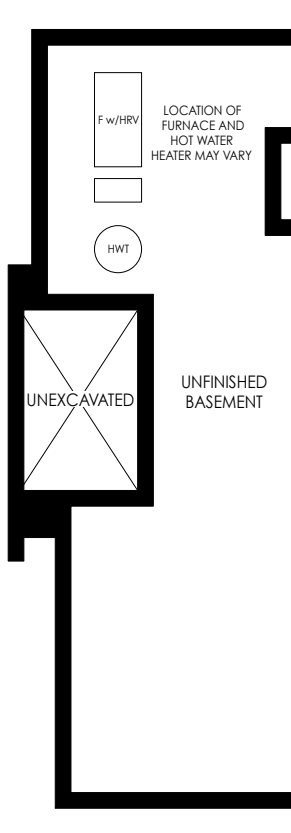
PARTIAL BASEMENT PLAN ELEV. 'M4'
