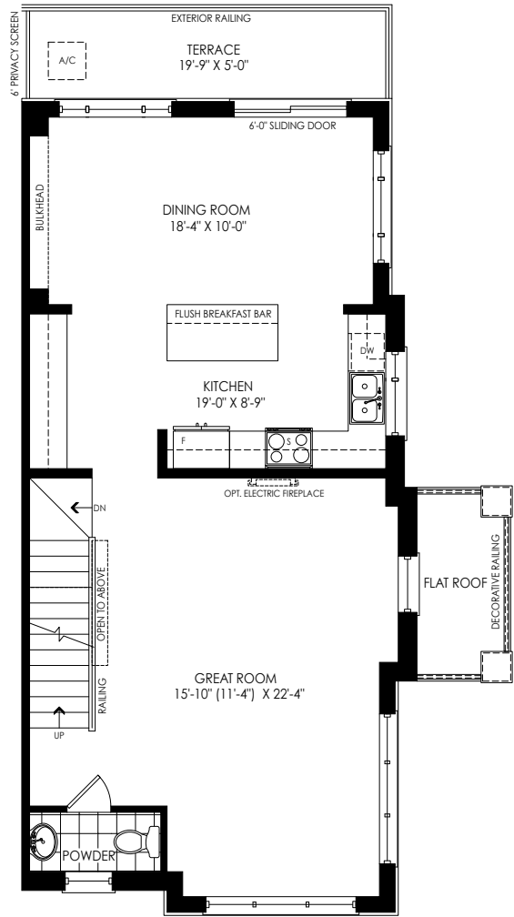
SECOND FLOOR PLAN ELEV. 'WC1'
