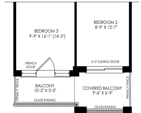
PARTIAL SECOND FLOOR PLAN ELEV 'M1'
