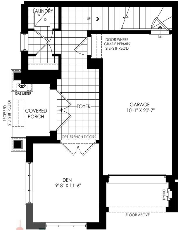
GROUND FLOOR PLAN ELEV. 'FC4'
