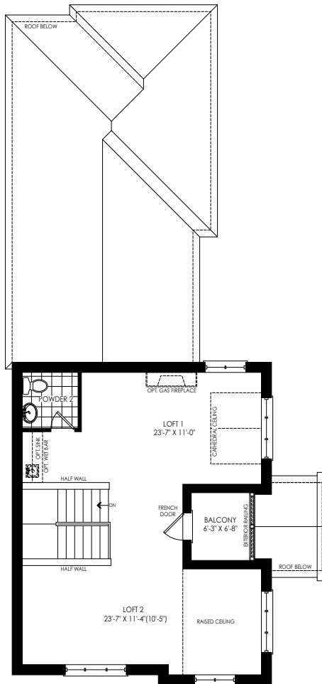
LOFT PLAN ELEV. 'E'
