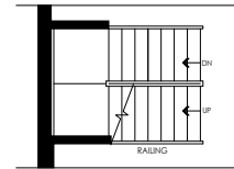
PARTIAL GROUND FLOOR PLAN FOR OPT. FINISHED BASEMENT LANDING ELEV. 'D'
