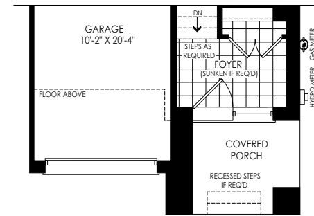
PARTIAL GROUND FLOOR PLAN ELEV 'WC5'
