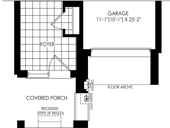
PARTIAL GROUND FLOOR PLAN ELEV. 'M1'
