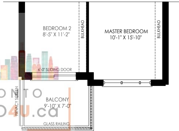
PARTIAL THIRD FLOOR PLAN ELEV. 'M1'
