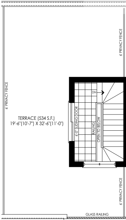
ROOF TERRACE PLAN ELEV. 'M1'
