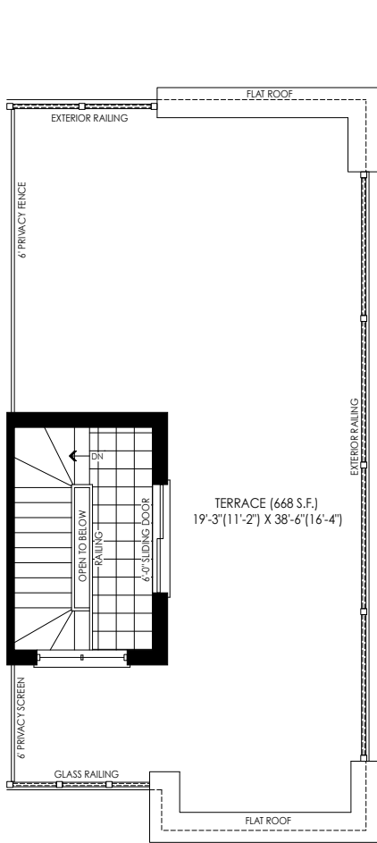
ROOF TERRACE PLAN ELEV. 'WC1'
