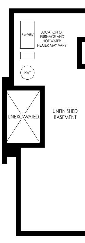
PARTIAL BASEMENT PLAN ELEV. 'WC5'
