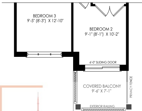
PARTIAL SECOND FLOOR PLAN ELEV 'T4'
