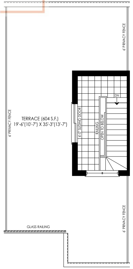
ROOF TERRACE PLAN ELEV. 'M1'
