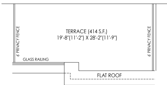
PARTIAL ROOF TERRACE PLAN ELEV. 'WC1'
