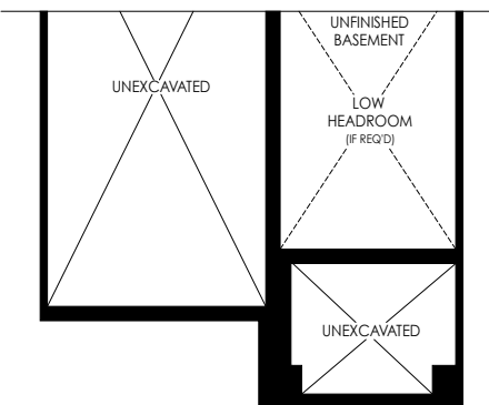
PARTIAL BASEMENT PLAN ELEV 'M3'
