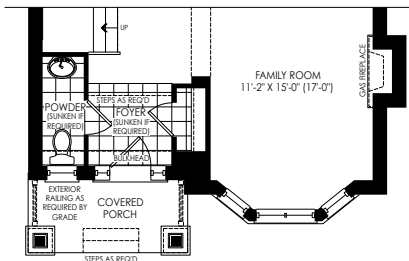
PARTIAL GROUND FLOOR PLAN ELEV. 'B'
