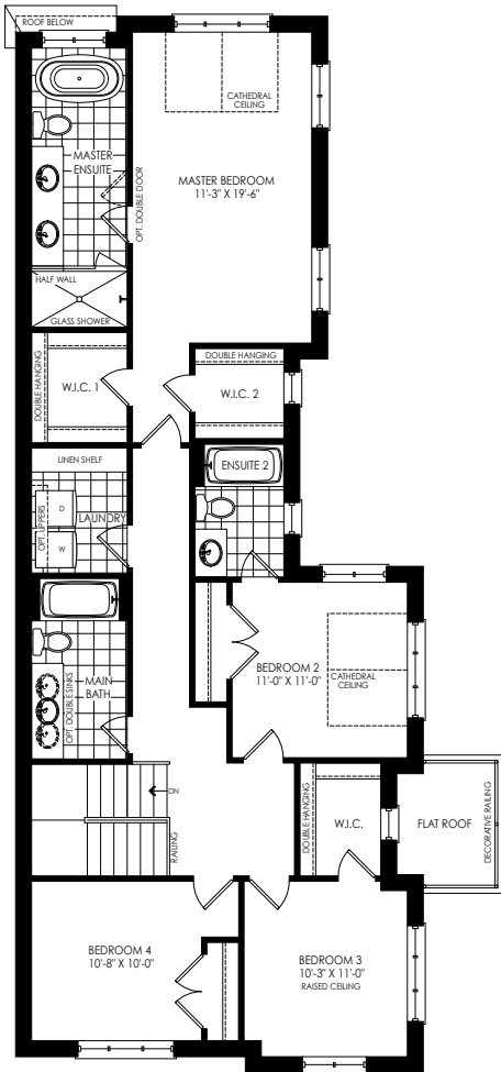
SECOND FLOOR PLAN ELEV. 'E'
