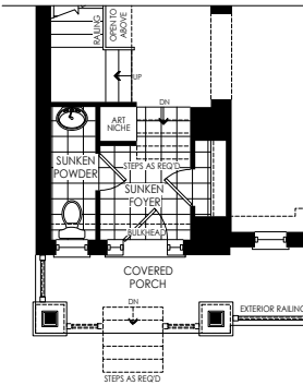
PARTIAL GROUND FLOOR PLAN ELEV. 'B' W/ SUNKEN FOYER CONDITION
