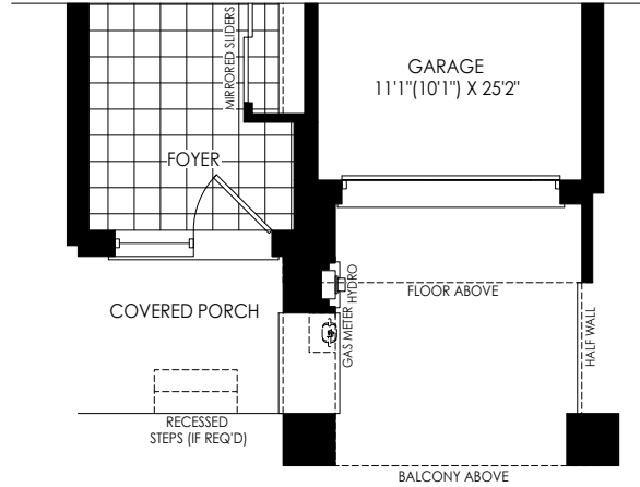
PARTIAL GROUND FLOOR PLAN ELEV. 'WC1' & 'WC2'
