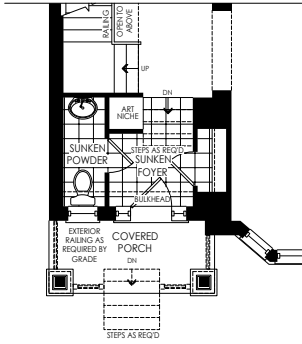
PARTIAL GROUND FLOOR PLAN ELEV. 'D' W/ SUNKEN FOYER CONDITION
