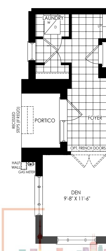
PARTIAL GROUND FLOOR PLAN ELEV. 'M4'
