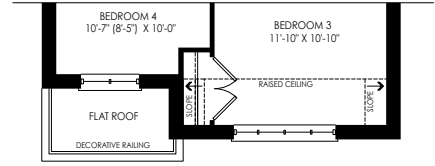
PARTIAL SECOND FLOOR PLAN ELEV. 'E'
