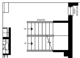
PARTIAL GROUND FLOOR PLAN FOR OPT. FINISHED BASEMENT LANDING ELEV. 'C', 'A' & 'E'
