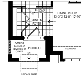
PARTIAL GROUND FLOOR PLAN ELEV. 'E' W/ SUNKEN FOYER CONDITION
