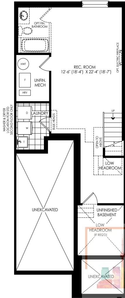
BASEMENT PLAN ELEV 'T1'
