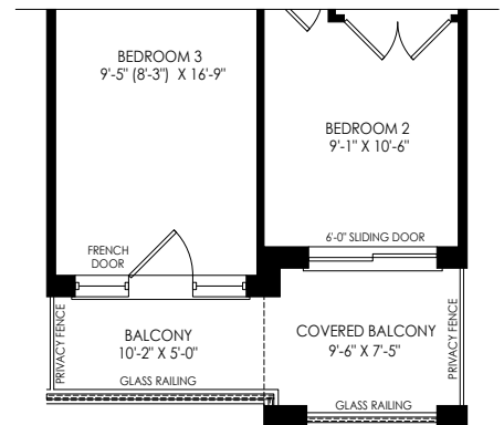
PARTIAL SECOND FLOOR PLAN ELEV 'M1'
