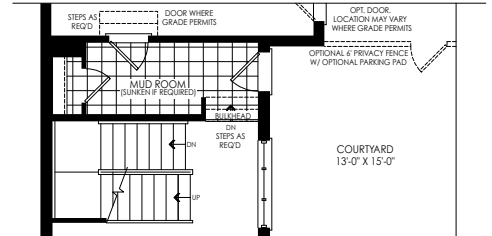
PARTIAL GROUND FLOOR PLAN FOR OPT. FINISHED BASEMENT LANDING ELEV. 'D'
