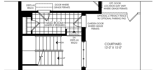
PARTIAL GROUND FLOOR PLAN FOR OPT. FINISHED BASEMENT LANDING ELEV. 'A' & 'B'
