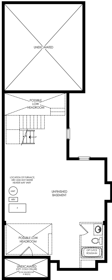
BASEMENT PLAN ELEV. 'D'
