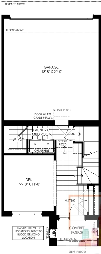
GROUND FLOOR PLAN ELEV. 'WC1'
