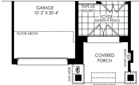
PARTIAL GROUND FLOOR PLAN ELEV 'T2' & 'T4'
