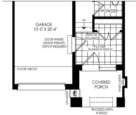
PARTIAL GROUND FLOOR PLAN ELEV 'M2'
