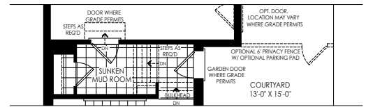
PARTIAL GROUND FLOOR PLAN ELEV. 'D', 'A' & 'B' W/ SUNKEN MUD ROOM CONDITION
