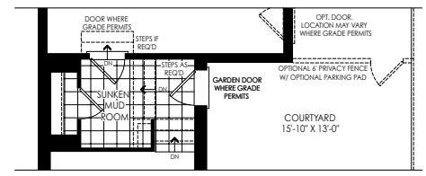
PARTIAL GROUND FLOOR PLAN ELEV. 'C', 'A' & 'E' W/ SUNKEN MUD ROOM CONDITION
