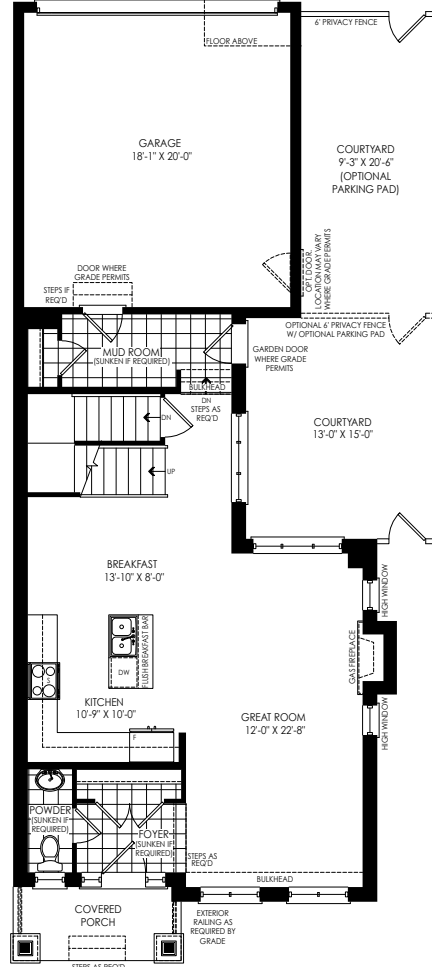
GROUND FLOOR PLAN ELEV. 'B'
