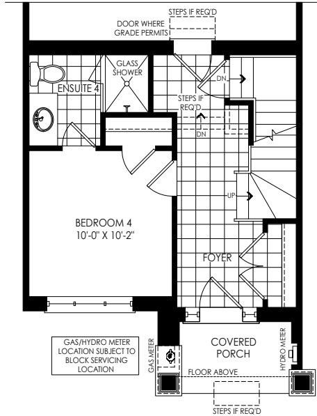
PARTIAL OPT. GROUND FLOOR PLAN W/ 4 BEDROOMS ELEV. 'F1' & 'FC1'
