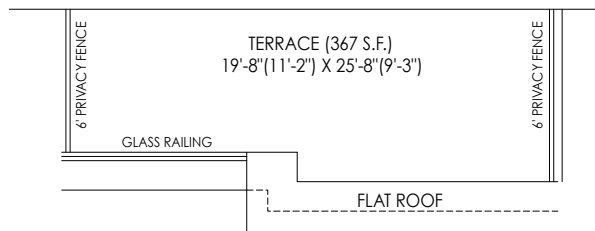
PARTIAL ROOF TERRACE PLAN ELEV. 'WC2'
