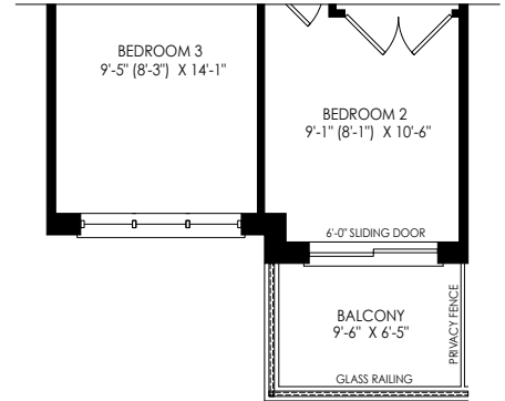
PARTIAL SECOND FLOOR PLAN ELEV 'M2'
