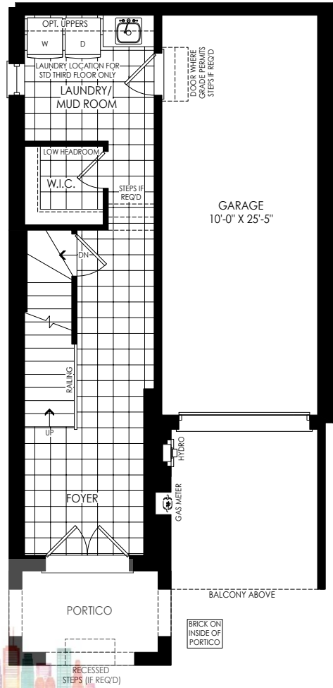
GROUND FLOOR PLAN ELEV. 'FC3'
