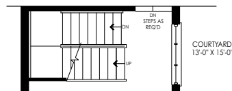
PARTIAL GROUND FLOOR PLAN FOR OPT. FINISHED BASEMENT LANDING ELEV. 'D'
