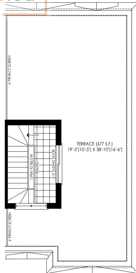
ROOF TERRACE PLAN ELEV. 'FC1'
