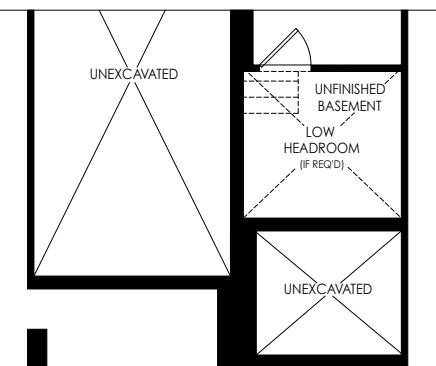
PARTIAL BASEMENT PLAN ELEV 'WC1' & 'WC2'
