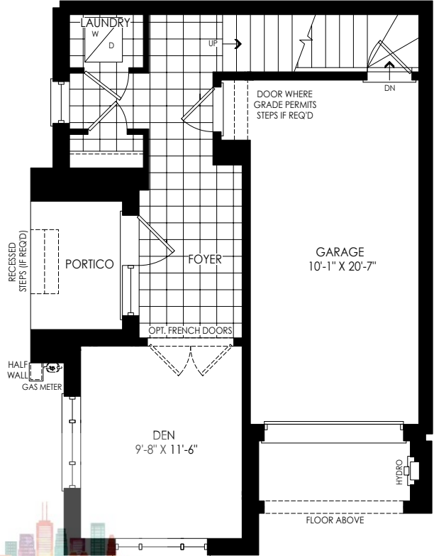
GROUND FLOOR PLAN ELEV. 'M3'
