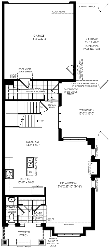
GROUND FLOOR PLAN ELEV. 'D'
