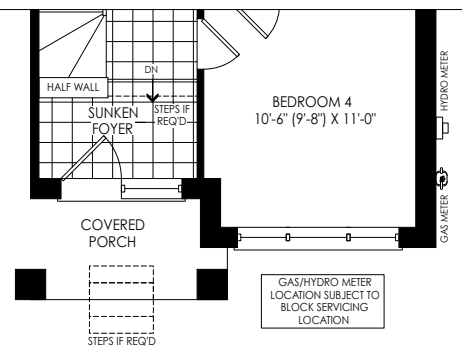
PARTIAL OPT. GROUND FLOOR PLAN W/ 4 BEDROOMS ELEV. 'WC1' W/ SUNKEN FOYER CONDITION
