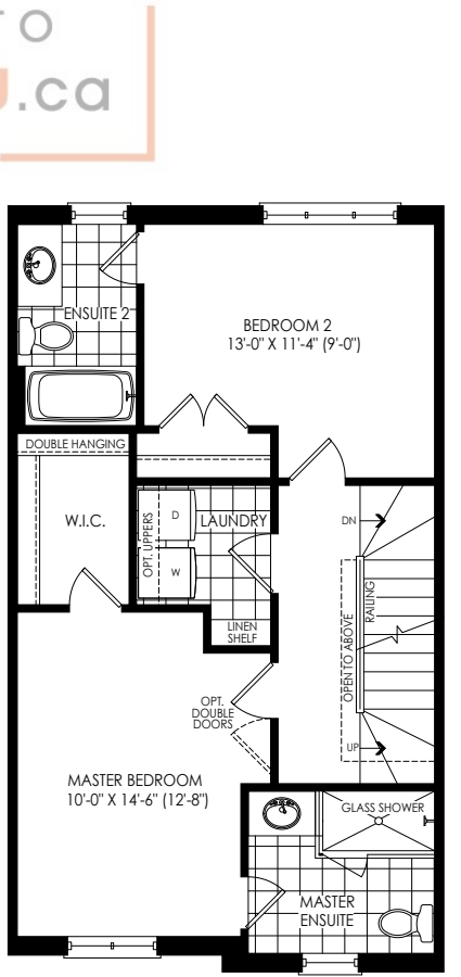
THIRD FLOOR PLAN ELEV. 'F1'
