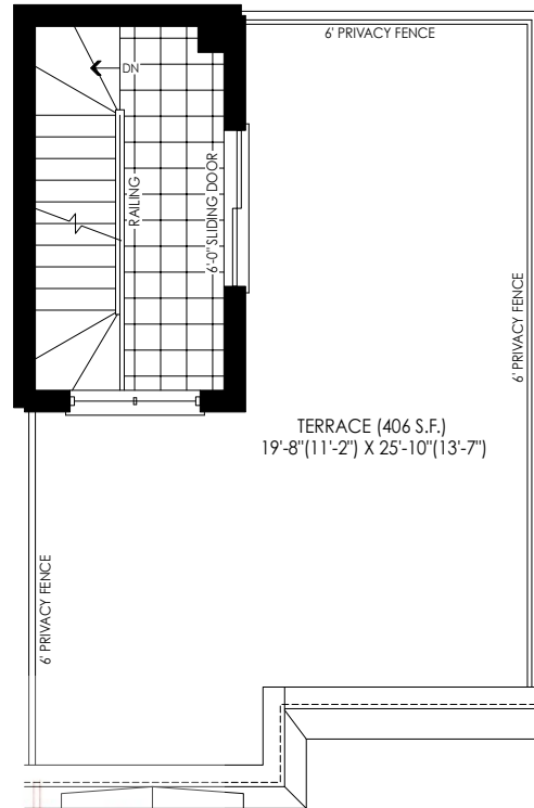
ROOF TERRACE PLAN ELEV. 'FC1'
