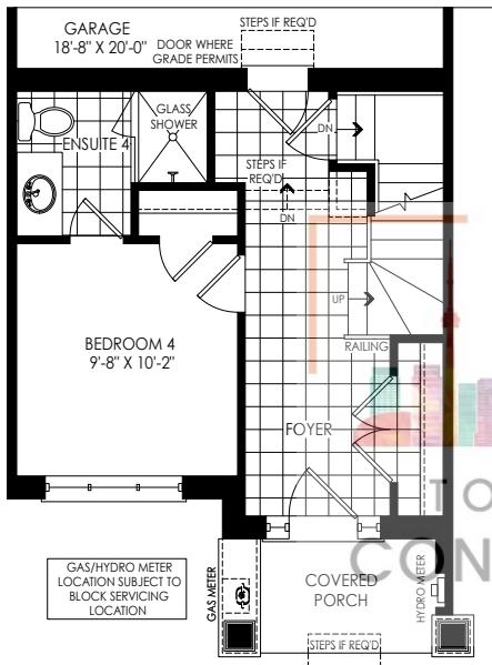
PARTIAL OPT. GROUND FLOOR PLAN W/ 4 BEDROOMS ELEV. 'F1' & 'FC1'
