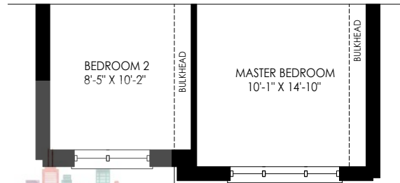
PARTIAL THIRD FLOOR PLAN ELEV. 'WC1' & 'WC2'
