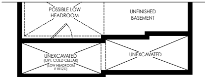
PARTIAL BASEMENT PLAN ELEV. 'B'
