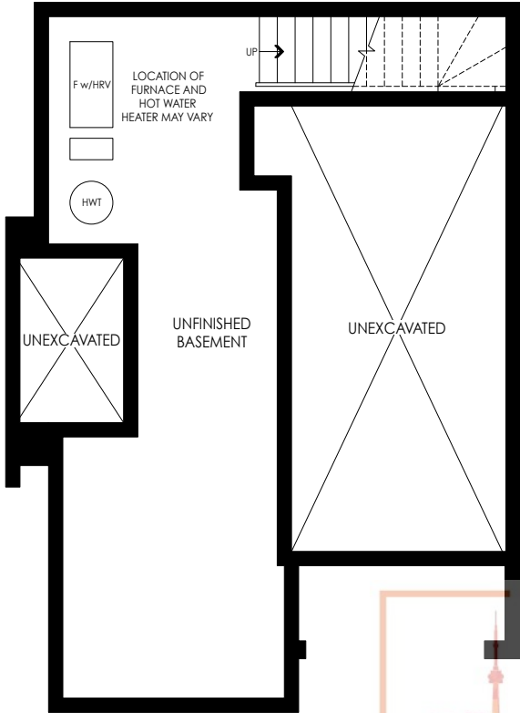
BASEMENT PLAN ELEV. 'WC4'
