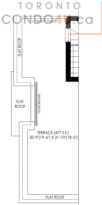
PARTIAL ROOF TERRACE PLAN ELEV. 'WC5'
