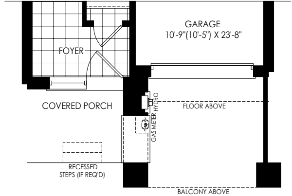
PARTIAL GROUND FLOOR PLAN ELEV. 'WC1' & 'WC2'
