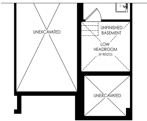
PARTIAL BASEMENT PLAN ELEV 'M1'
