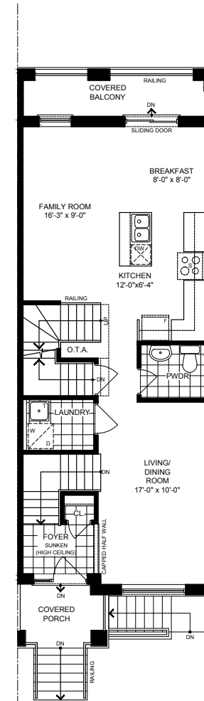
MAIN FLOOR PLAN
