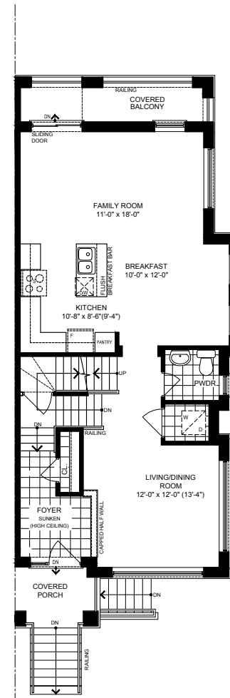
MAIN FLOOR PLAN
