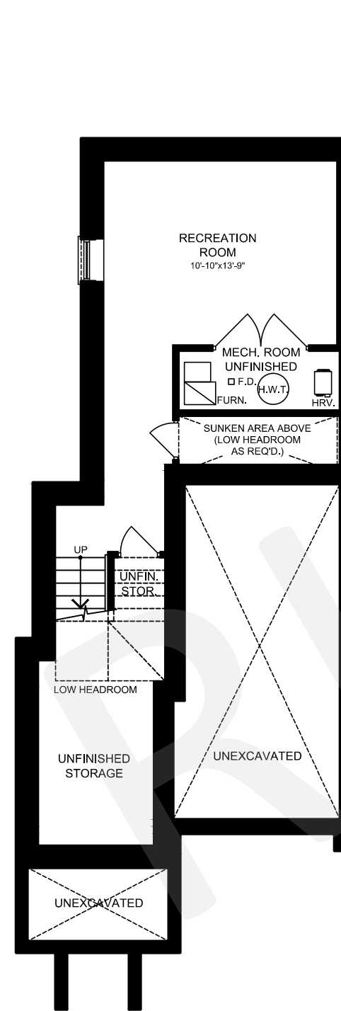
ELEV. A Basement
